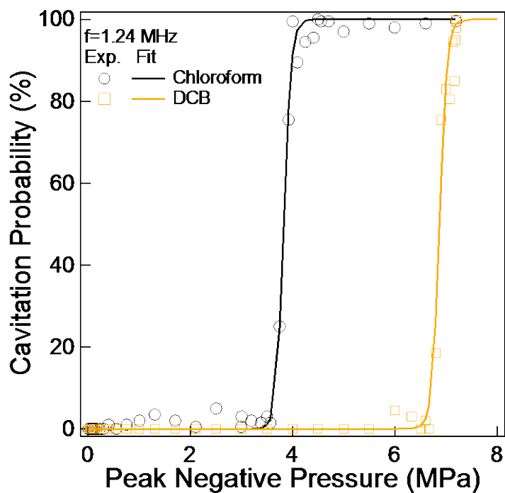
Figure S8. Cavitation probability of solvents as a function of peak negative pressure for chloroform and dichlorobenzene.
