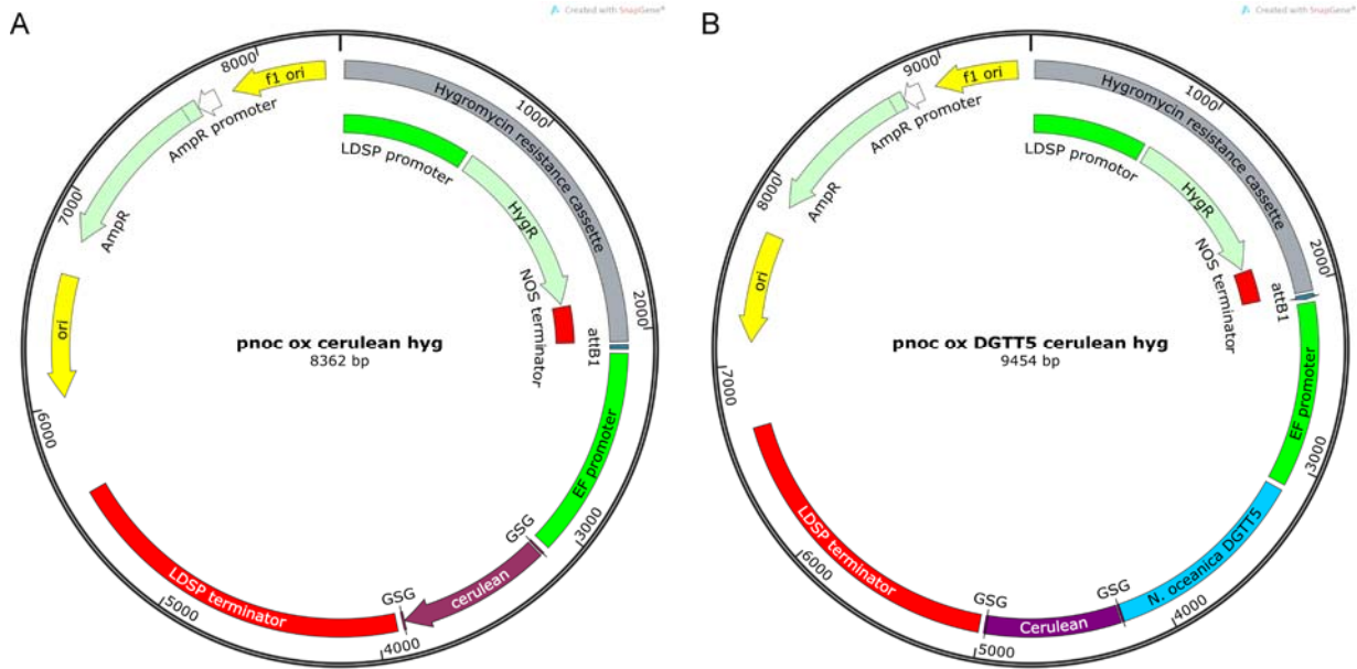
Figure S5. Maps of the plasmids used for the generation of N. oceanica DGTT5 -overexpressing strains. A, pnoc ox cerulean hyg vector control. B, pnoc ox DGTT5 cerulean hyg for overexpressing DGTT5 .
