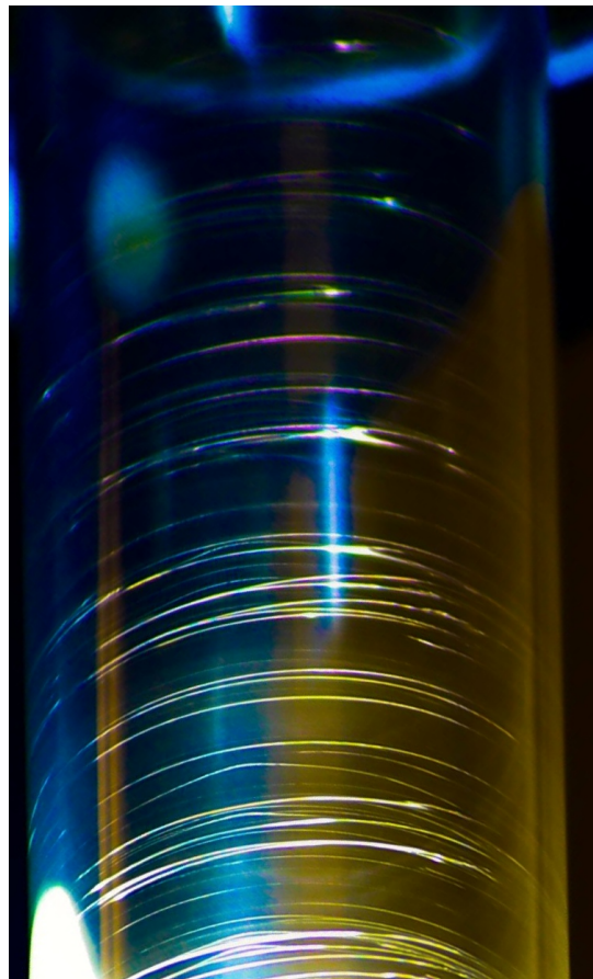
Figure S2 An enlarged longitudinal photograph of a Faraday wave present in the VFD. The contrast of the image has been adjusted to enhance clarity of the waves.
