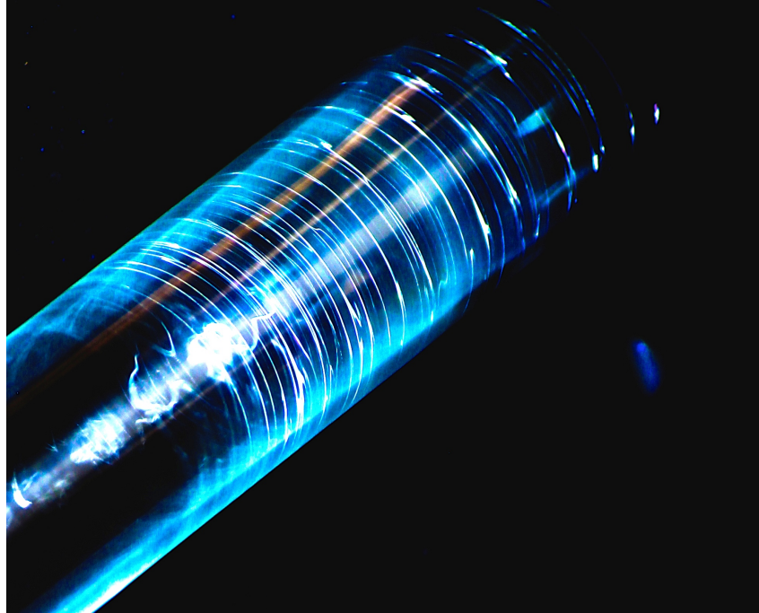
Figure S1 A photograph of Faraday waves present in the VFD. The contrast of the image has been adjusted to enhance clarity.
