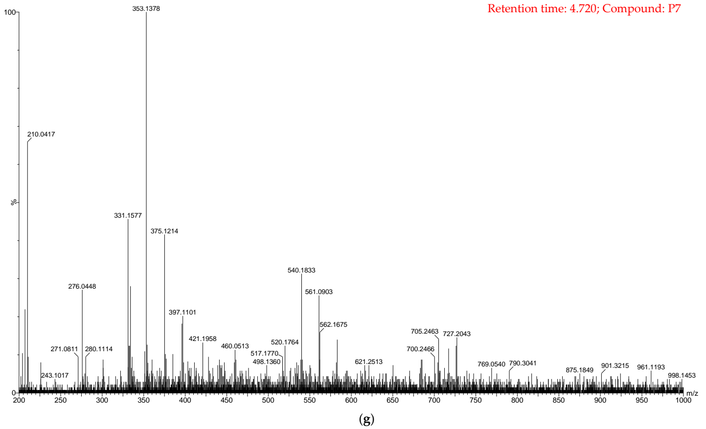
Figure S1. The corresponding mass spectrum data of seven peaks with retention times at 1.471 min (a), 1.590 min (b), 1.796 min (c), 2.103 min (d), 2.736 min (e), 4.087 min (f), and 4.720 min (g).
