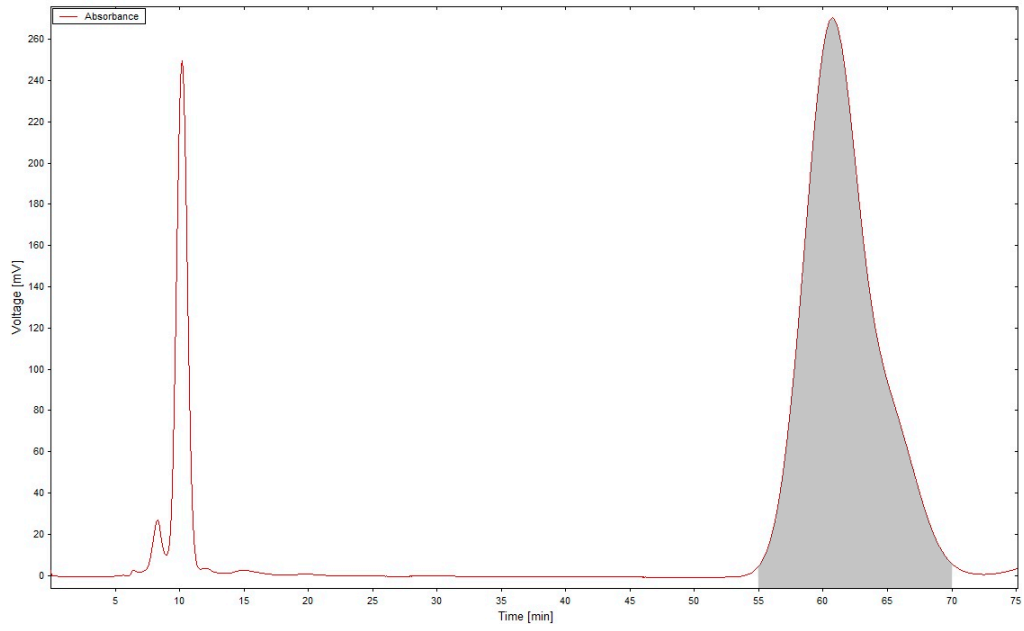
Figure S1. HPCCC chromatogram of N. damascena essential oil.
