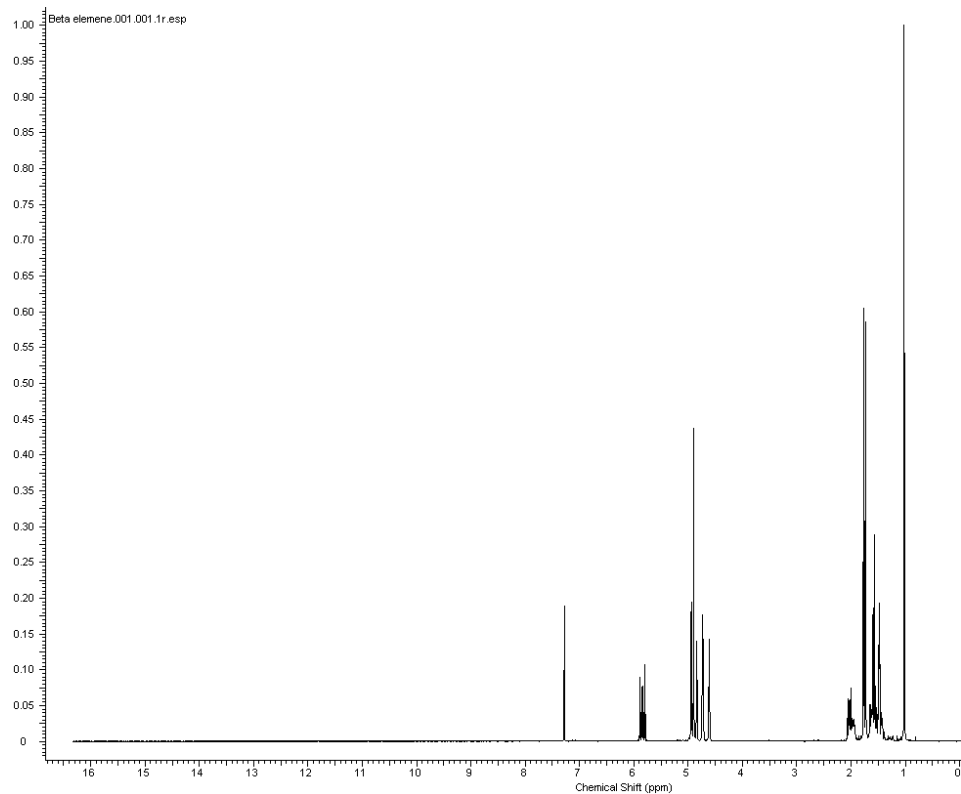
Figure S3: ^1\text{H} NMR spectrum of \beta -elemene.
