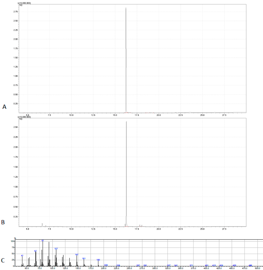
Figure S2 A: GC chromatogram of N. damascena essential oil, B: GC chromatogram of \beta -elemene standard, C: GC chromatogram of isolated \beta -elemene, D: MS spectrum of \beta -elemene;
