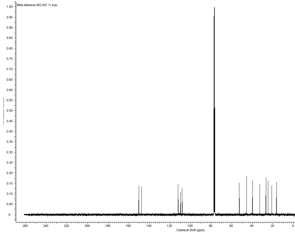
Figure S4: ^{13}\text{C} NMR spectrum of \beta -elemene.
