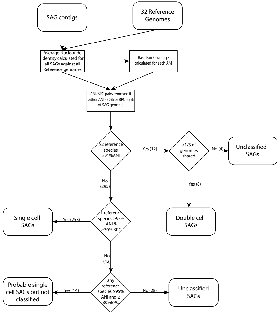
Supplemental Figure 3. Schematic overview of the logic pipeline used to classify single amplified genomes (SAG). The average nucleotide identity (ANI) was calculated using the script provided here ( https://github.com/chjp/ANI ) and the base pair coverage (BPC) was calculated using a custom perl script. Numbers in parenthesis indicate the number of SAGs at each step of the pipeline.
