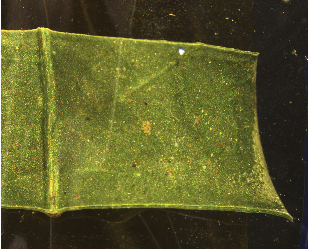
Supplementary Figure 1. Bright-field light microscopy image of the Glochidion sericeum leaf from Figures 3–4.
