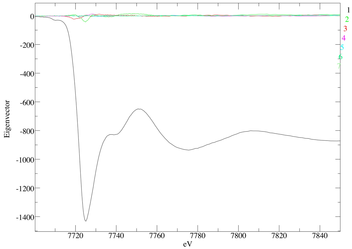
Supplementary Figure 5. Principal Component Analysis of Co K-edge X-ray spectra of different samples of G. sericeum leaves and other tissues show in Fig 8.
