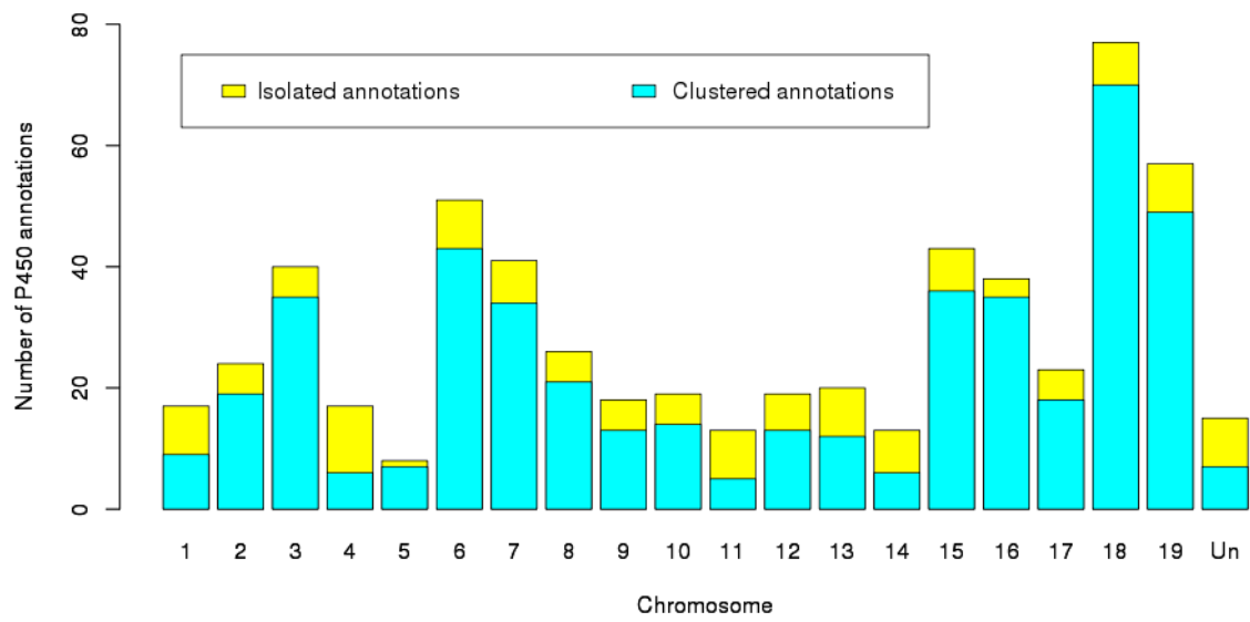
S3 Fig. Distribution of the V. vinifera P450s per chromosome. The blue bar corresponds to clustered annotations and the yellow bar to the isolated annotations. The “Unknown chromosome” is labeled as “Un”.
