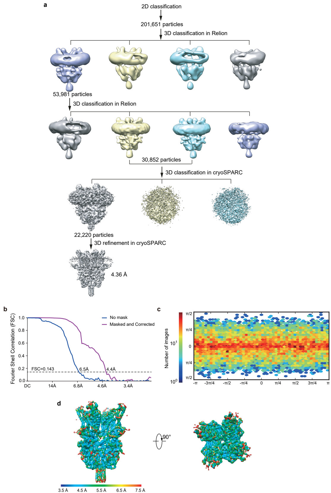
Figure S8. Cryo-EM image analysis of the hTRPC3 channel in nanodiscs.
