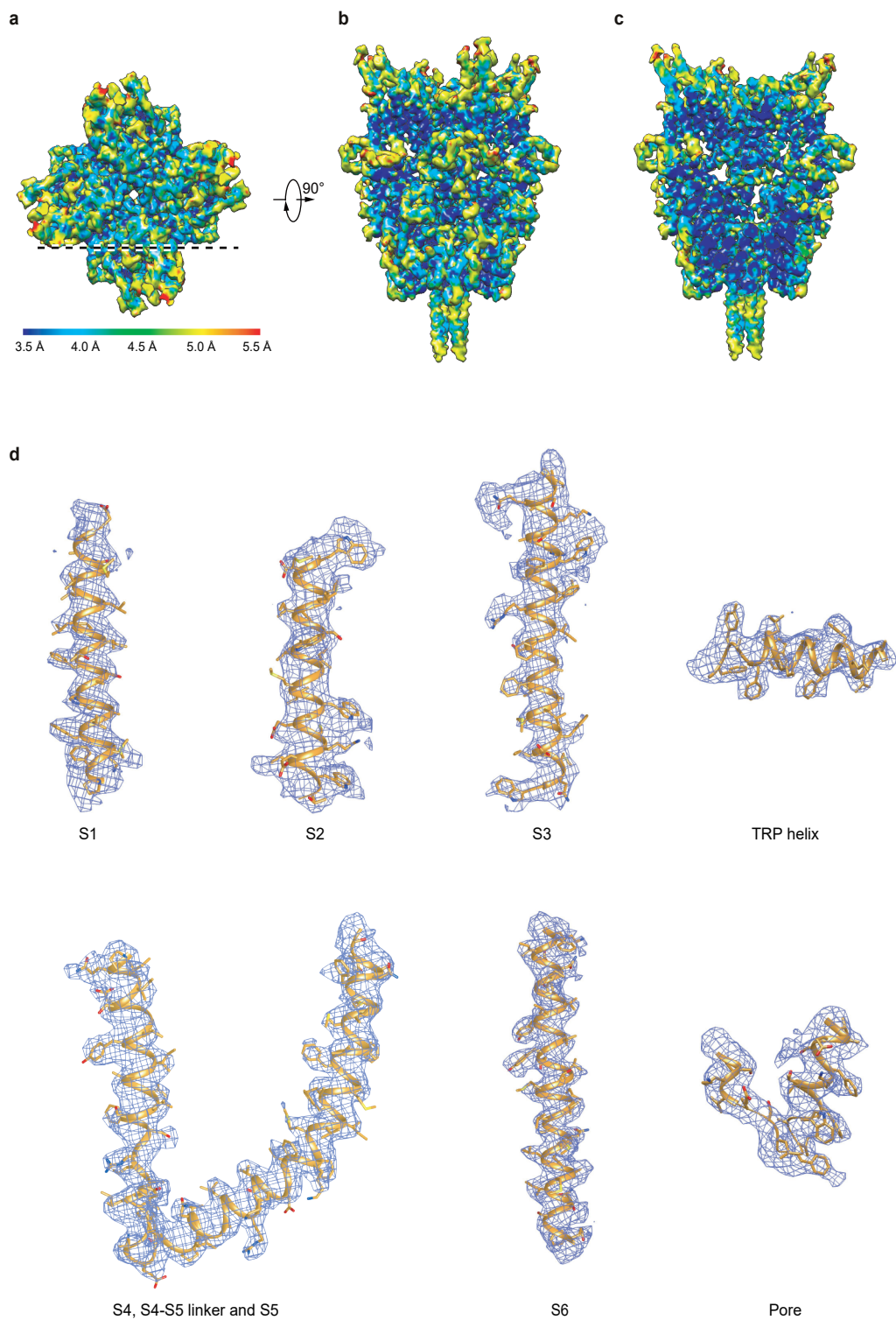
Figure S3. Cryo-EM map of hTRPC6 in nanodiscs.
