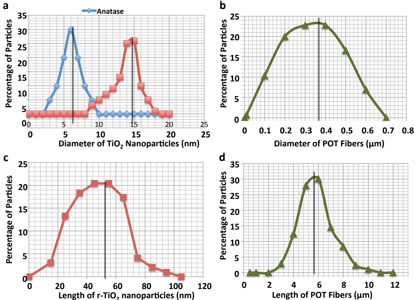
Figure S1. Diameters of a-nTiO 2 and r-nTiO 2 (a) and POT fibers (b). Lengths of r-nTiO 2 (c) and POT fibers (d).
