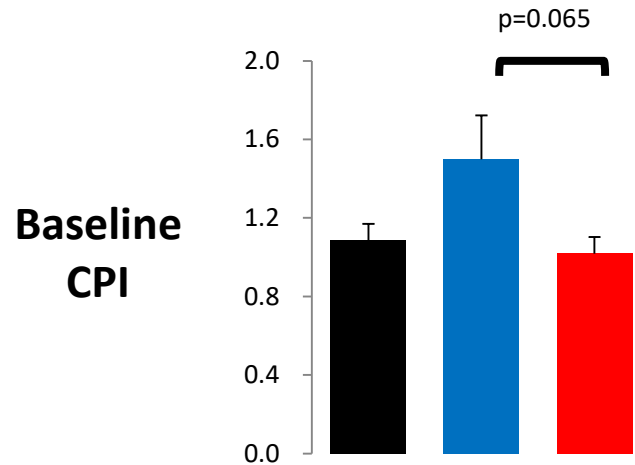
Figure S1. Comparison of C-peptide index (CPI) between patients with HbA1c <7% and those with HbA1c ≥7% at 54 weeks in 49 patients, including 12 who were originally excluded due to receiving additional OADs or bolus insulin. Black bar, all subjects (n=49); Blue bar, patients with HbA1c <7% at 54 weeks (n=7); and Red bar, patients with HbA1c ≥7% at 54 weeks or those receiving additional OADs or bolus insulin during the 54 weeks (n=42). Each value represents the mean ± SEM. A P-value was calculated by the Mann-Whitney U-test.
