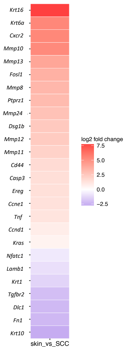
Malignancy markers Tumor vs Skin
