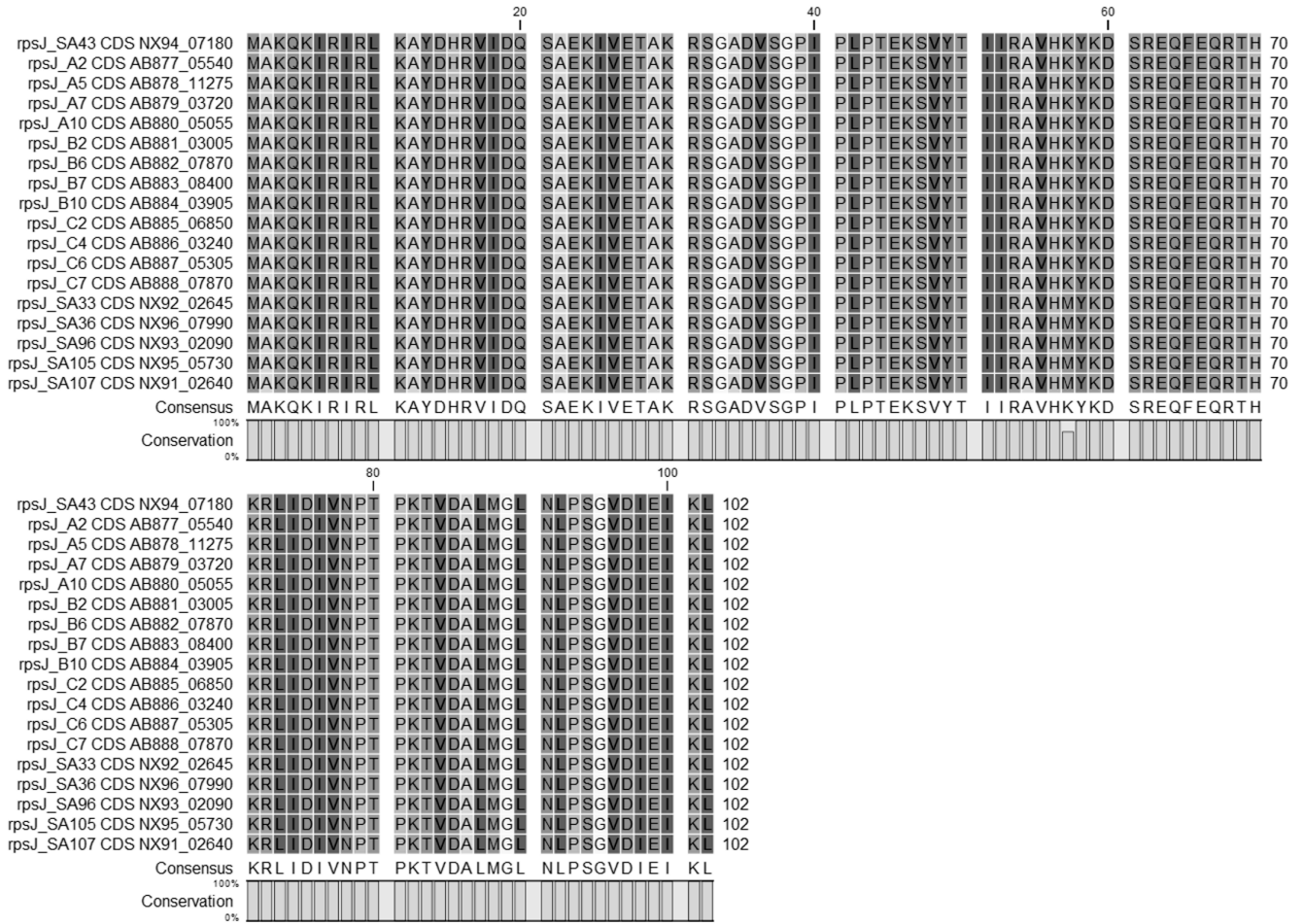
Figure S1 – Alignment of the S10 protein sequence showing the K57M amino acid substitution in the clinical MRSA TGC-S strains SA33, SA36, SA96, SA105 and SA107 (MIC = 0.25 mg/L).
