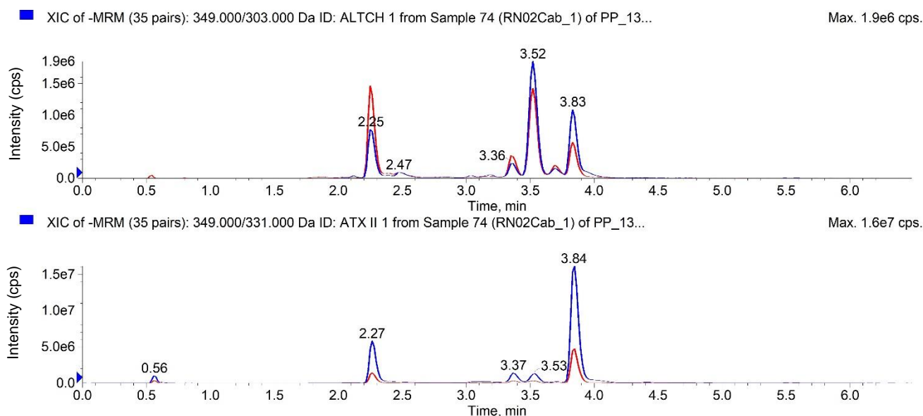
Figure-S1: Extracted ion chromatogram of alterperlylenol (above) and altertoxin-II (below)
