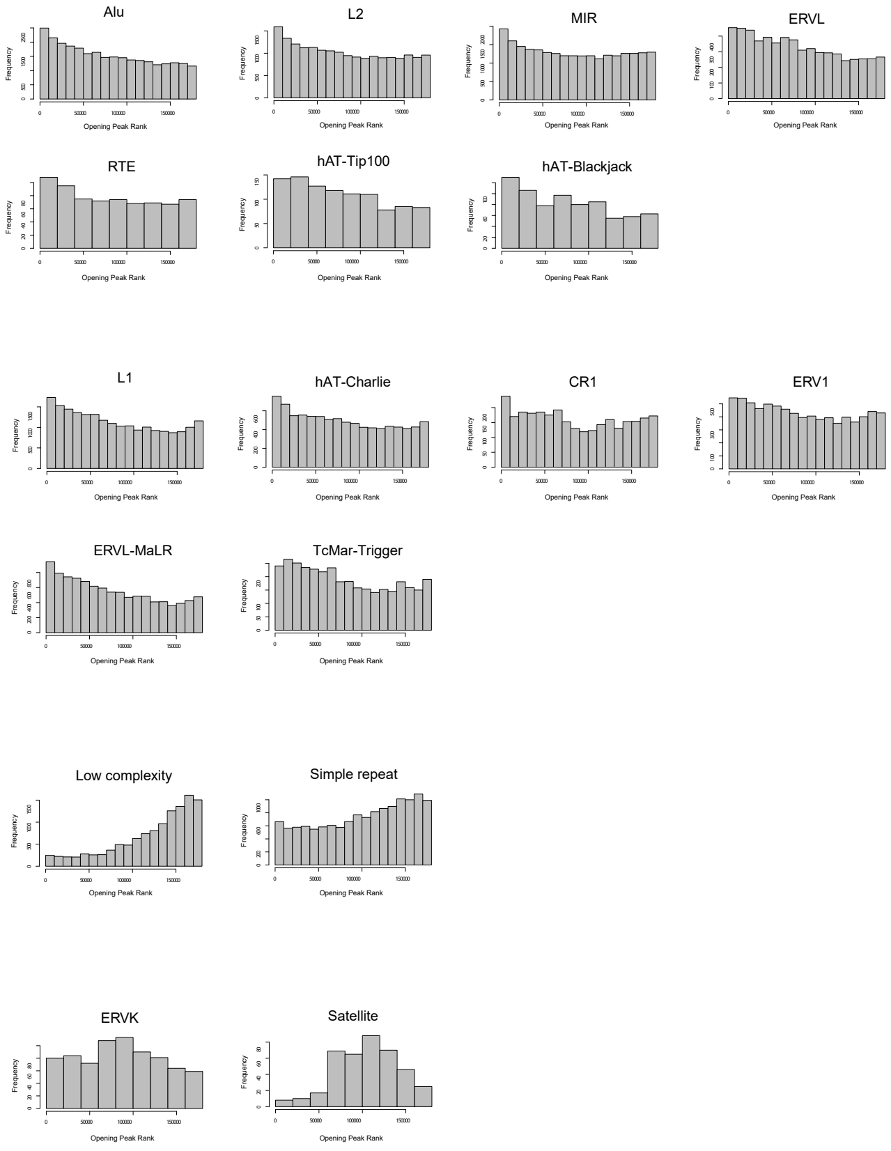
Figure S8. Association of other repetitive elements with opening and closing of chromatin (expansion of Figure 5B).
