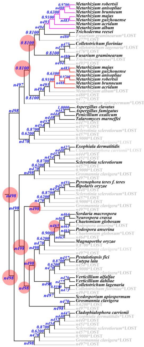
S6 Fig: Estimation of gene duplication and loss events of the Pks genes in the fungal species shown in Fig 1A by reconciling the raw Pks gene's ML tree (Fig 1A) with the species tree (S4 Fig) using NOTUNG with a duplication-loss (DL) model with default parameters (1.5 for duplication and 1.0 for loss), and six other parameter combinations (1.0 for duplication, 1.0 for loss; 2.0 for duplication, 1.0 for loss; 1.5 for duplication, 0.5 for loss; 1.5 for duplication, 1.5 for loss; 1.5 for duplication, 0.5 for loss; 1.5 for duplication, 1.5 for loss). The same result was produced from all assays, and the one with default parameters was presented here as a representative. Red circles indicate duplication events inferred by the reconciliation. Blue notes near the nodes denote the internal node species name. Gray branches (branch name with LOST): inferred loss events.
