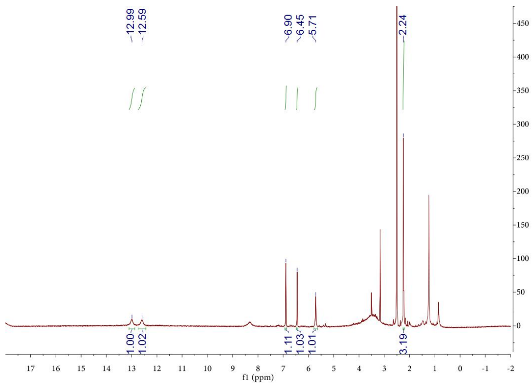
S17 Fig: ^1\text{H} NMR spectrum of Compound I (shown in Fig 8) in \text{DMSO-}d_6 .
