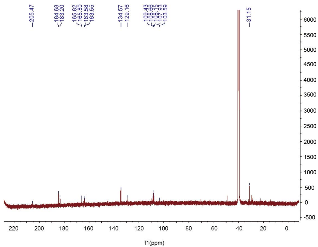
S18 Fig: ^{13}\text{C} NMR spectrum of Compound I (shown in Fig 8) in \text{DMSO-}d_6 .
