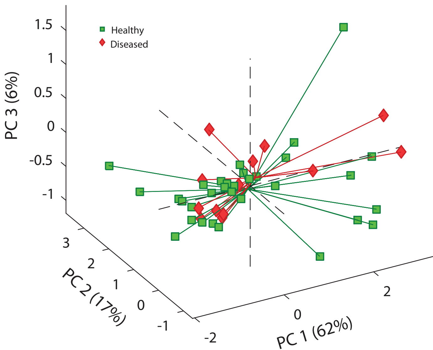
Principal component analysis of FT-NIR data. Score plot with three principal components.
