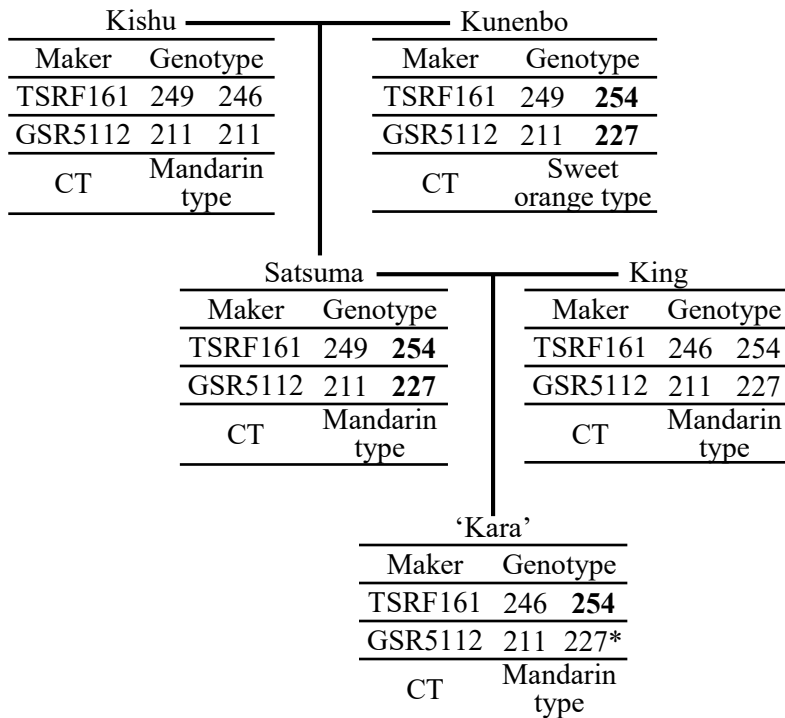
S4 Fig. Inheritance of the alleles of TSRF161 and GSR5112 linked with MS-PI in 'Kara' ancestors. Genotypes of simple sequence repeat markers and classes of organelle genotype (CT) were sourced from a previous report (Shimizu et al. 2016). The alleles derived from kunenbo are indicated in bold. *: Allele "227" at GSR5112 could not be estimated because the genotypes at GSR5112 were the same in Satsuma and King. CT: classes of organelle genotype.
