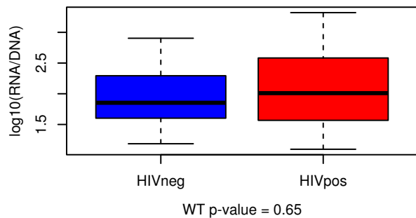
cutC_Choline TMA-Lyase
