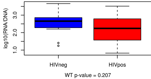
K01667_trypthophanase [EC:4.1.99.1]
