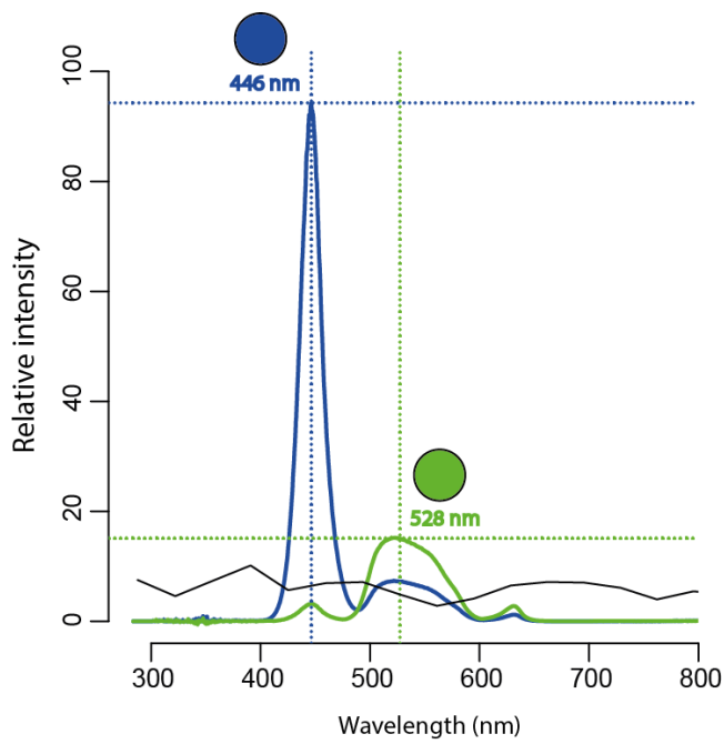
Figure S1. Spectral curves of the green (dominant wavelength 528 nm) and the blue disc (446 nm). The curve of the black background surrounding the colored discs is also shown (black curve). This curve slightly differs from a flat curve with a null intensity due to minimum amount of light produced by the videoprojector.
