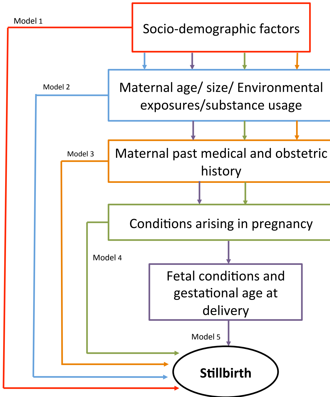
Figure S1: Hierarchical modelling strategy for the analysis of antepartum stillbirth risk factors
