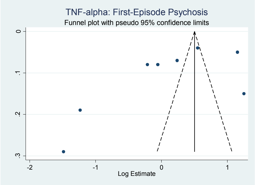
Supplementary Figure 2. Funnel plot of TNF- \alpha and First-Episode Psychosis
