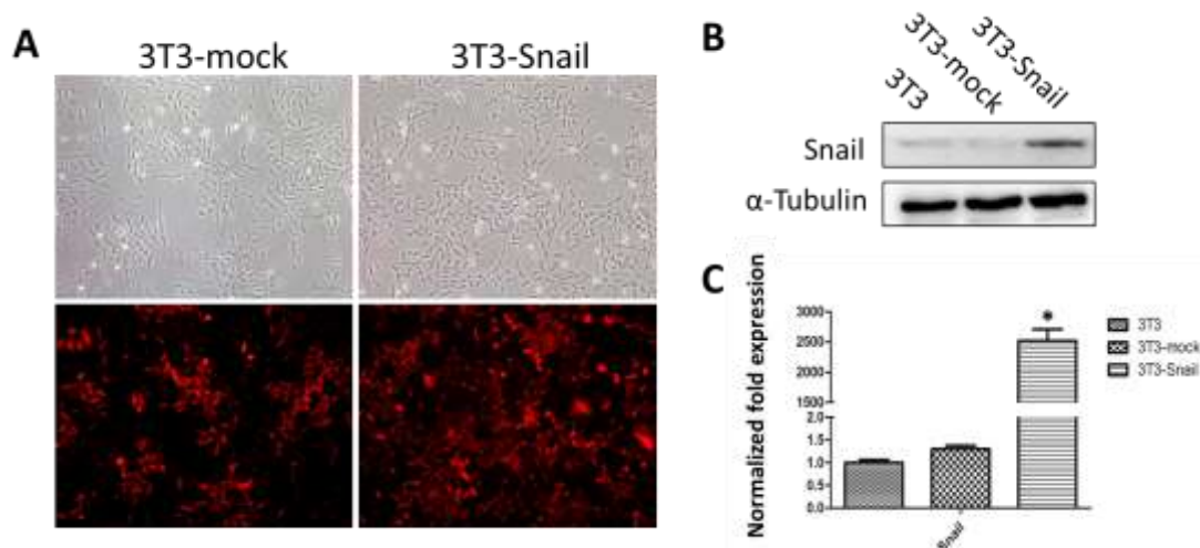
S1 Fig. Generation of stable over-expression of Snail 3T3 cell line (3T3-Snail). (A) White light and immunofluorescence images of the Snail or mock transduced 3T3 cells. (B) Snail expression in 3T3, 3T3-mock and 3T3-Snail stable cell lines were measured from total cell extracts by Western blot analysis. (C) The expression of Snail was detected by reverse transcription-quantitative polymerase chain reaction. Compared with control 3T3 and 3T3-mock cells, Snail expression levels were markedly upregulated in 3T3-Snail stable cell lines no matter in protein level or RNA level.
