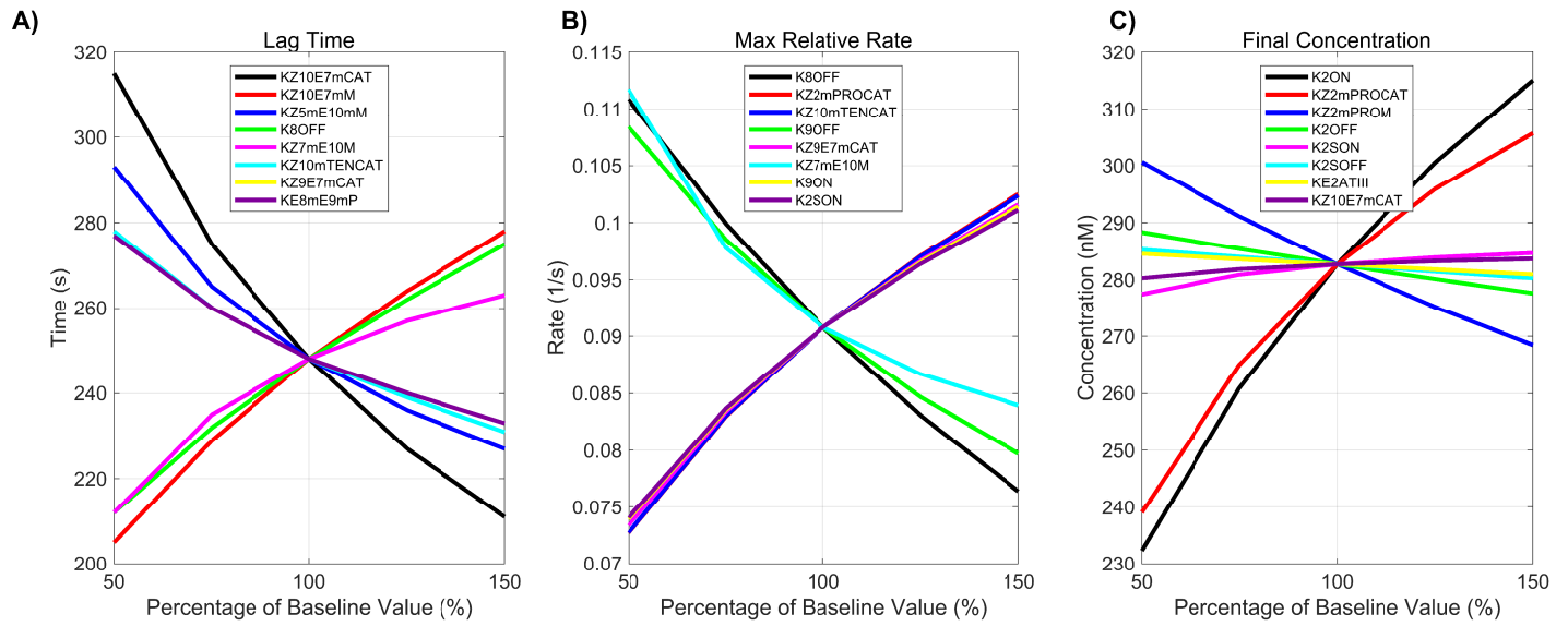
S1 Fig. Monotonicity of Change in Thrombin Generation due to Variation in KRCs. Variation in the three physiologically relevant metrics of thrombin generation: A) lag time; B) maximum relative rate of thrombin generation; 3) final concentration of thrombin: due to variations in the top eight model sensitive kinetic rate constants.
