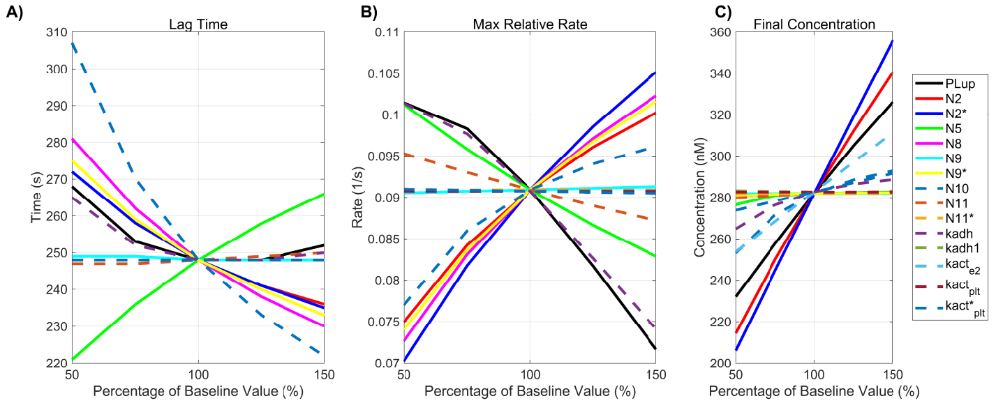
S2 Fig. Monotonicity of Change in Thrombin Generation due to Variation in PCs. Variation in the three physiologically relevant metrics of thrombin generation: A) lag time; B) maximum relative rate of thrombin generation; 3) final concentration of thrombin: due to variations in platelet characteristics.
