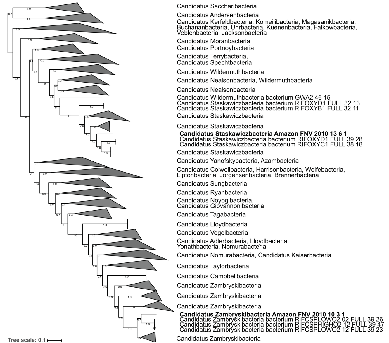
FIGURE S6 Maximum likelihood phylogenetic tree of 16 concatenated ribosomal proteins from superphylum Parcubacteria with Candidatus Saccharibacteria (TM7) as an outgroup, with 500 bootstrap replicates. The genomes from this study are indicated in bold. The numbers on each node represent the bootstrap support.
