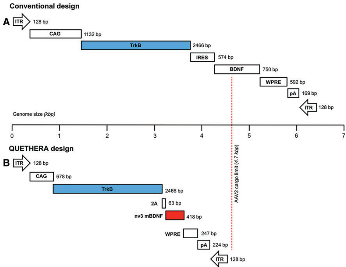
Supplementary Figure S1. (A) Schematic representation of the conventional elements necessary for production of TrkB and BDNF in an AAV2 vector system. (B) Schematic representation of elements used in the novel AAV2 TrkB-2A-mBDNF construct tested in this study. BDNF, brain-derived neurotrophic factor; ITR, inverted terminal repeat; IRES, Internal Ribosome Entry Site; mBDNF, mature BDNF; WPRE, woodchuck hepatitis virus posttranscriptional regulatory element; pA, polyadenylation sequence.
