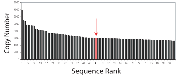
CDR3
