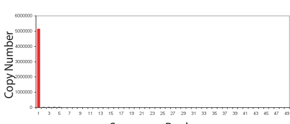
Sequence Rank
