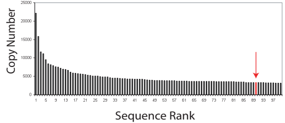
CDR3
