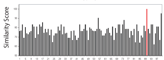
CDR3
