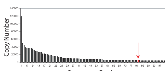
Sequence Rank
