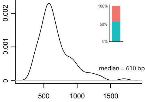
Highly recurrent genes (n=20)
