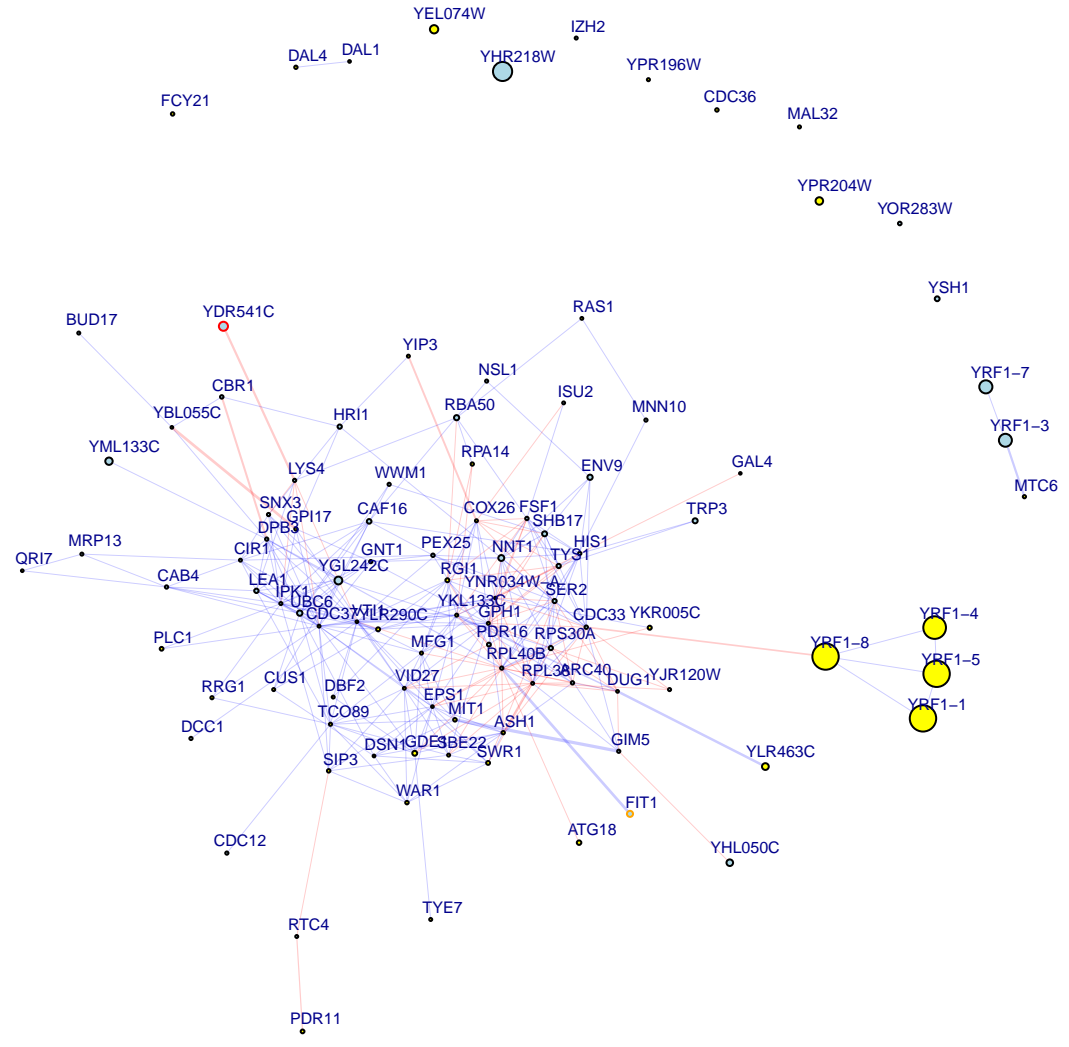
chrIV:1521369_A/C top 100 up and down genes
