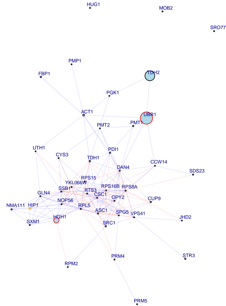
chrVII:850923_T/C top 50 up genes
