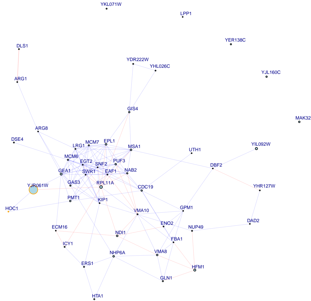
chrX:548174_T/C top 50 up genes
