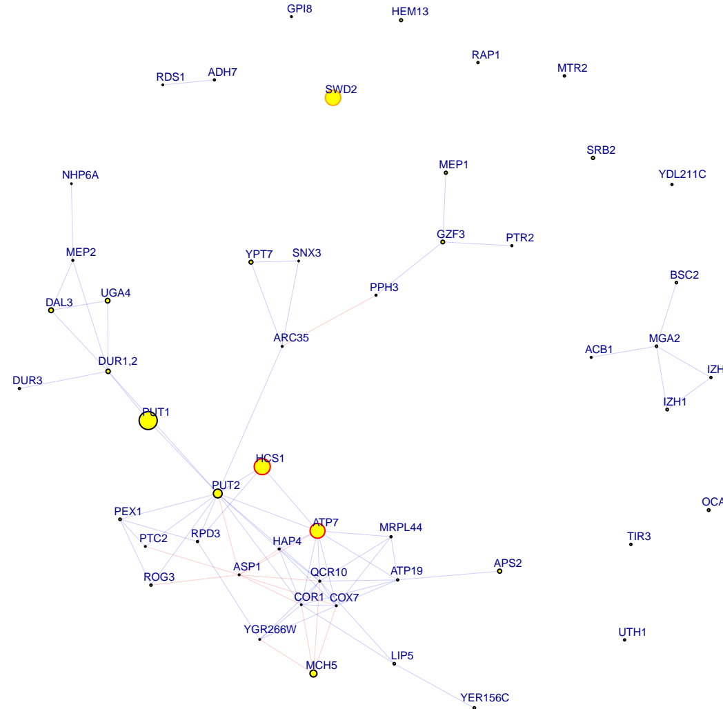
chrXI:411756_T/C top 50 down genes
