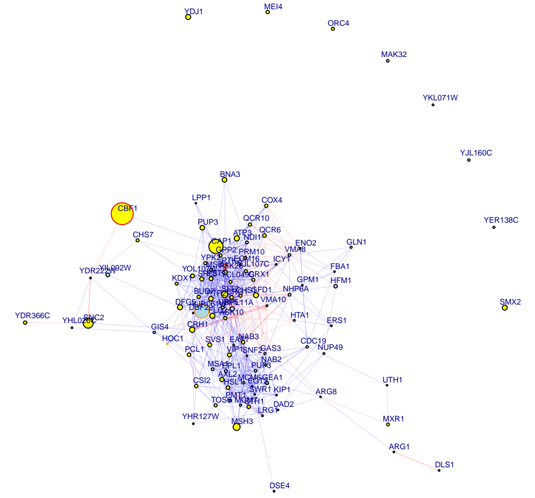
chrX:548174_T/C top 100 up and down genes
