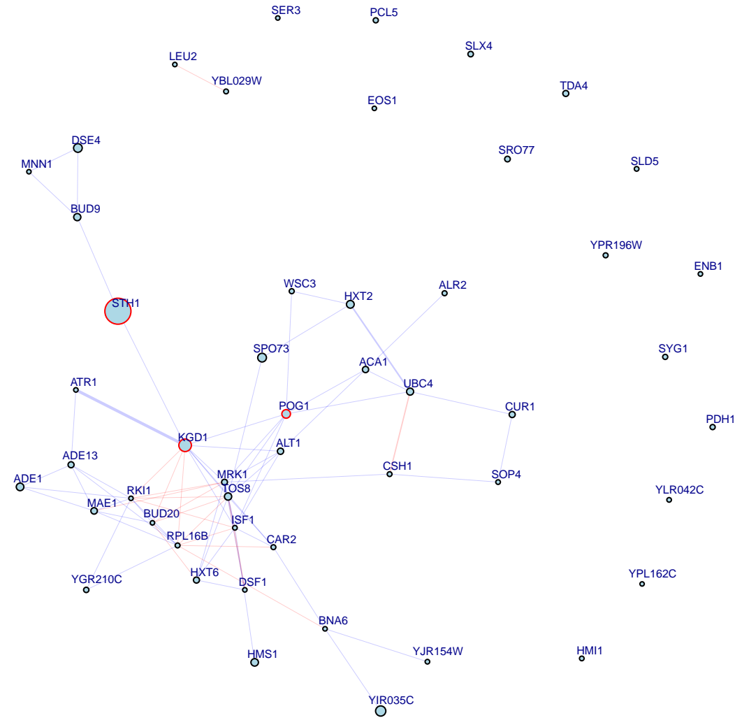
chrIX:105090_T/C top 50 up genes
