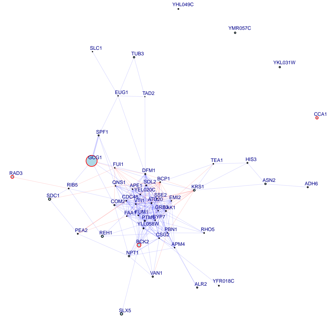
chrV:524625_A/T top 50 up genes
