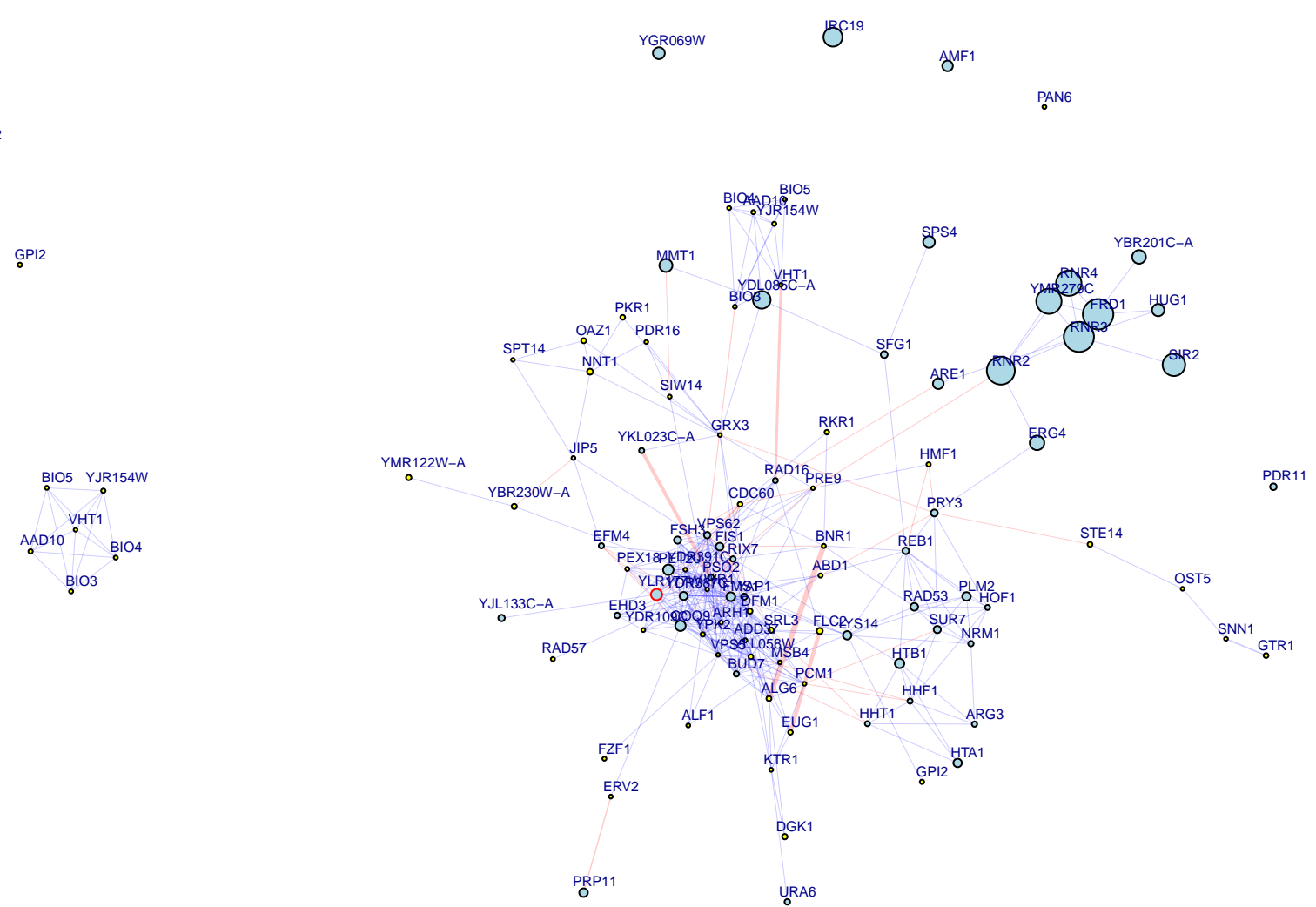
chrXII:510559_C/T top 100 up and down genes
