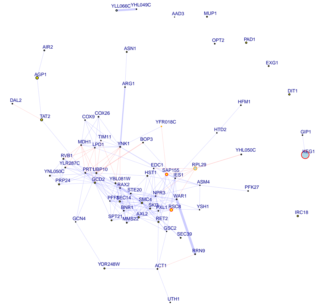
chrVI:229337_G/A top 66 up and down genes
