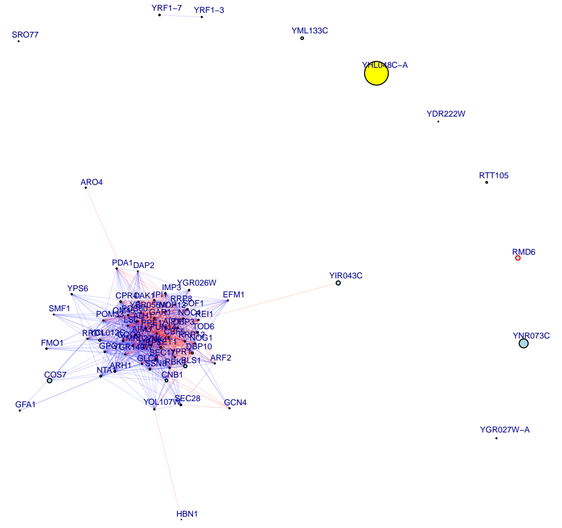
chrV:11186_T/C top 70 up and down genes
