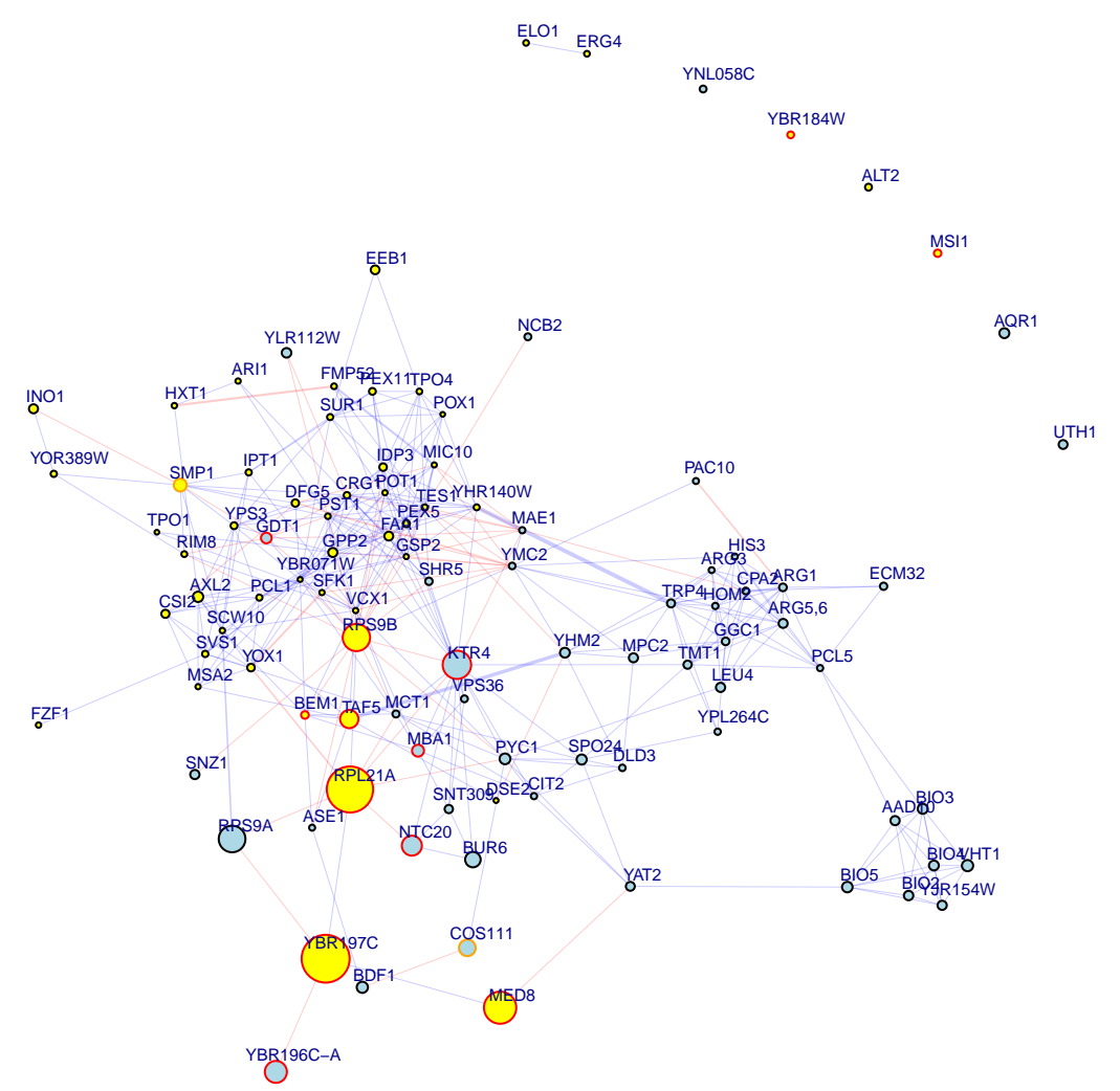
chrII:619028_C/A top 100 up and down genes
