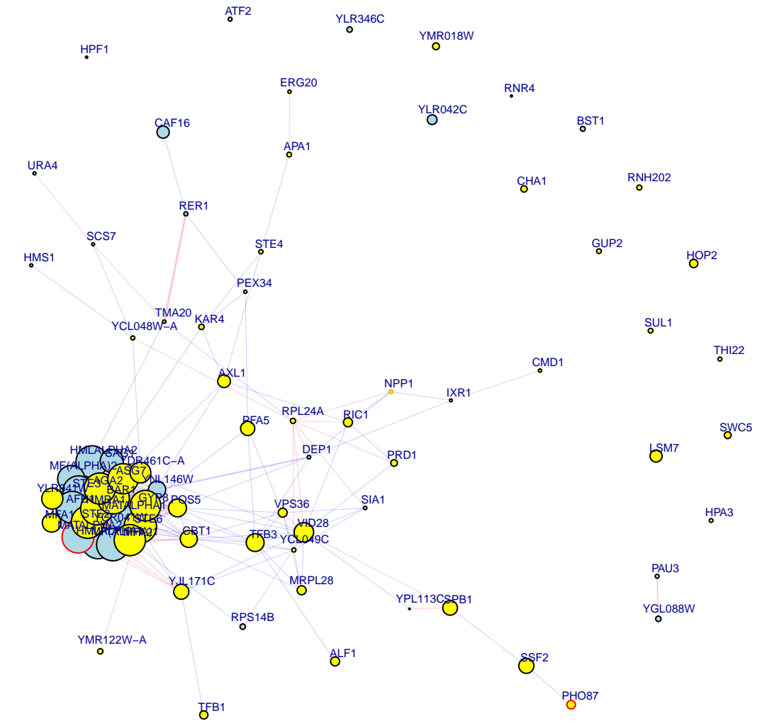
chrIII:201185_C/A top 78 up and down genes
