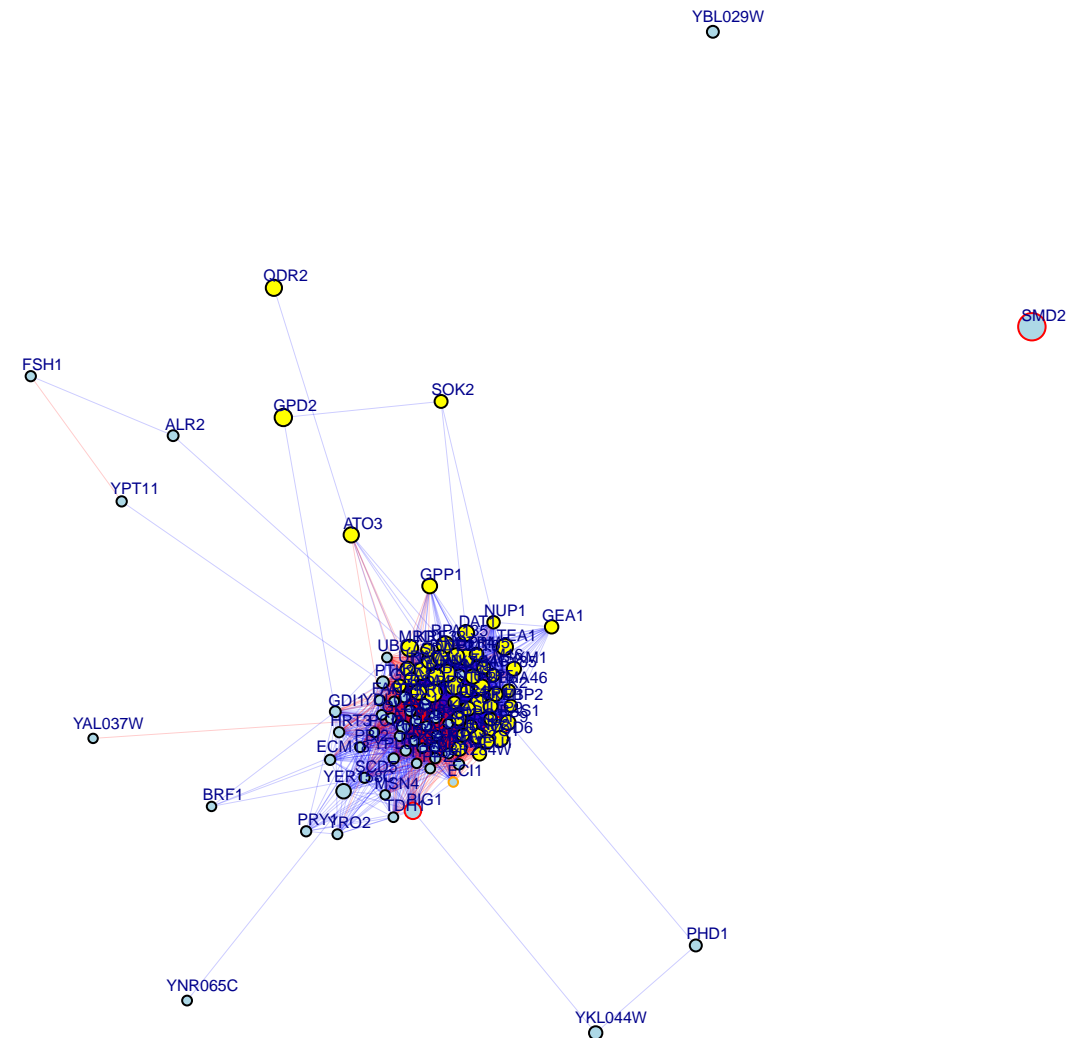
chrXII:694841_T/C top 100 up and down genes
