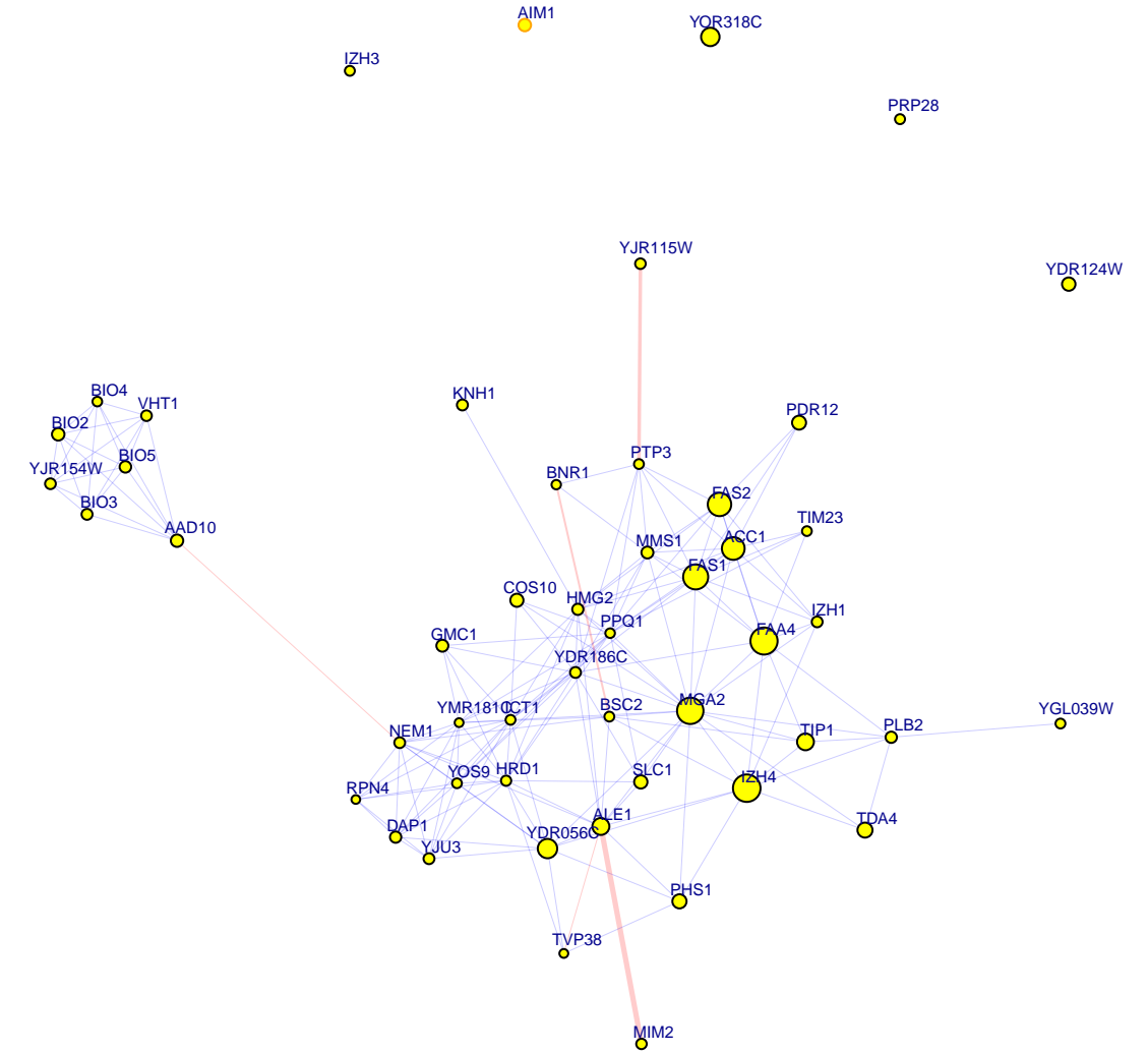
chr1:48890_C/T top 50 down genes
