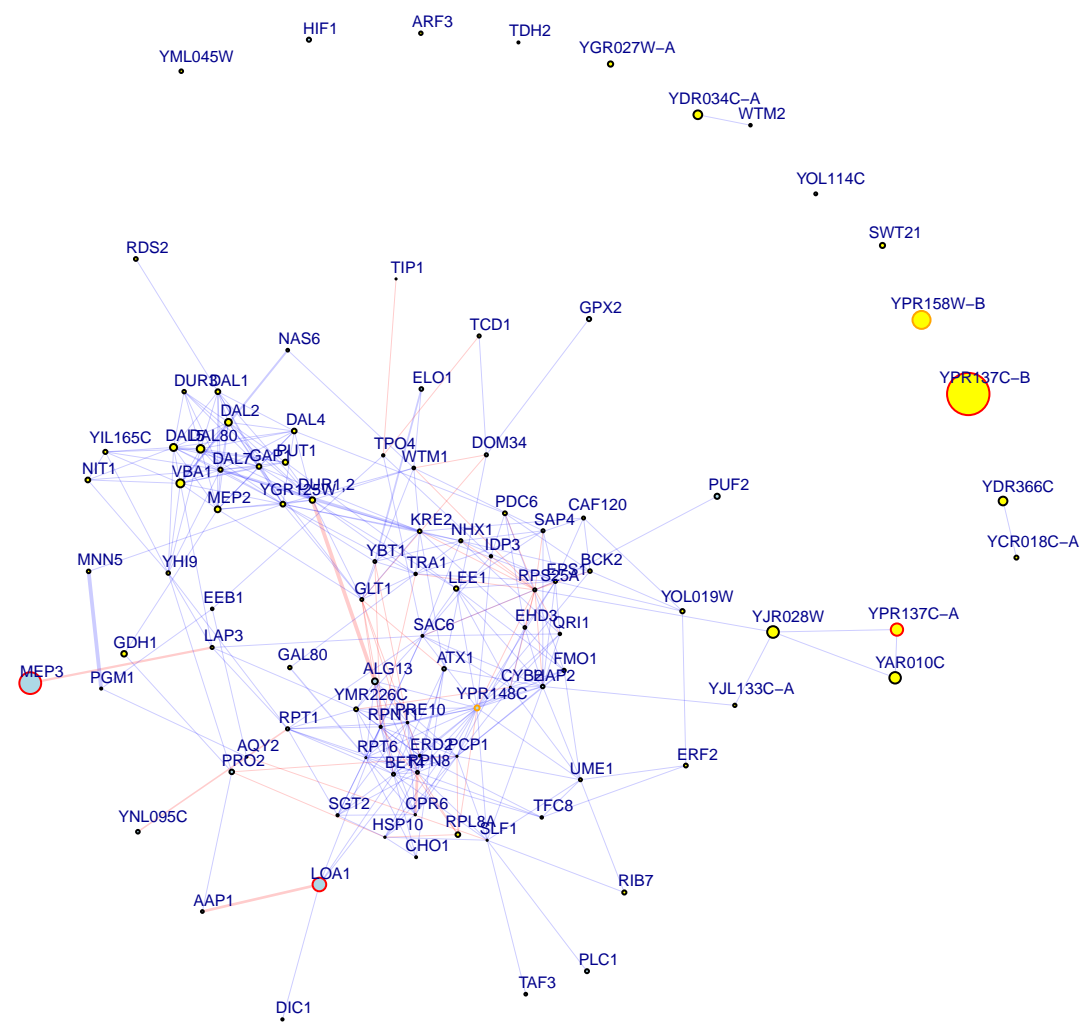
chrXVI:812990_T/C top 100 up and down genes
