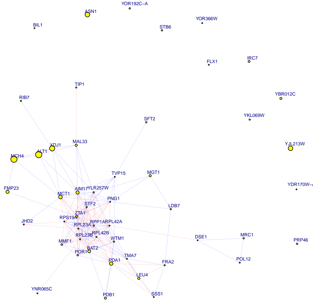
chrXV:958080_T/A top 50 down genes
