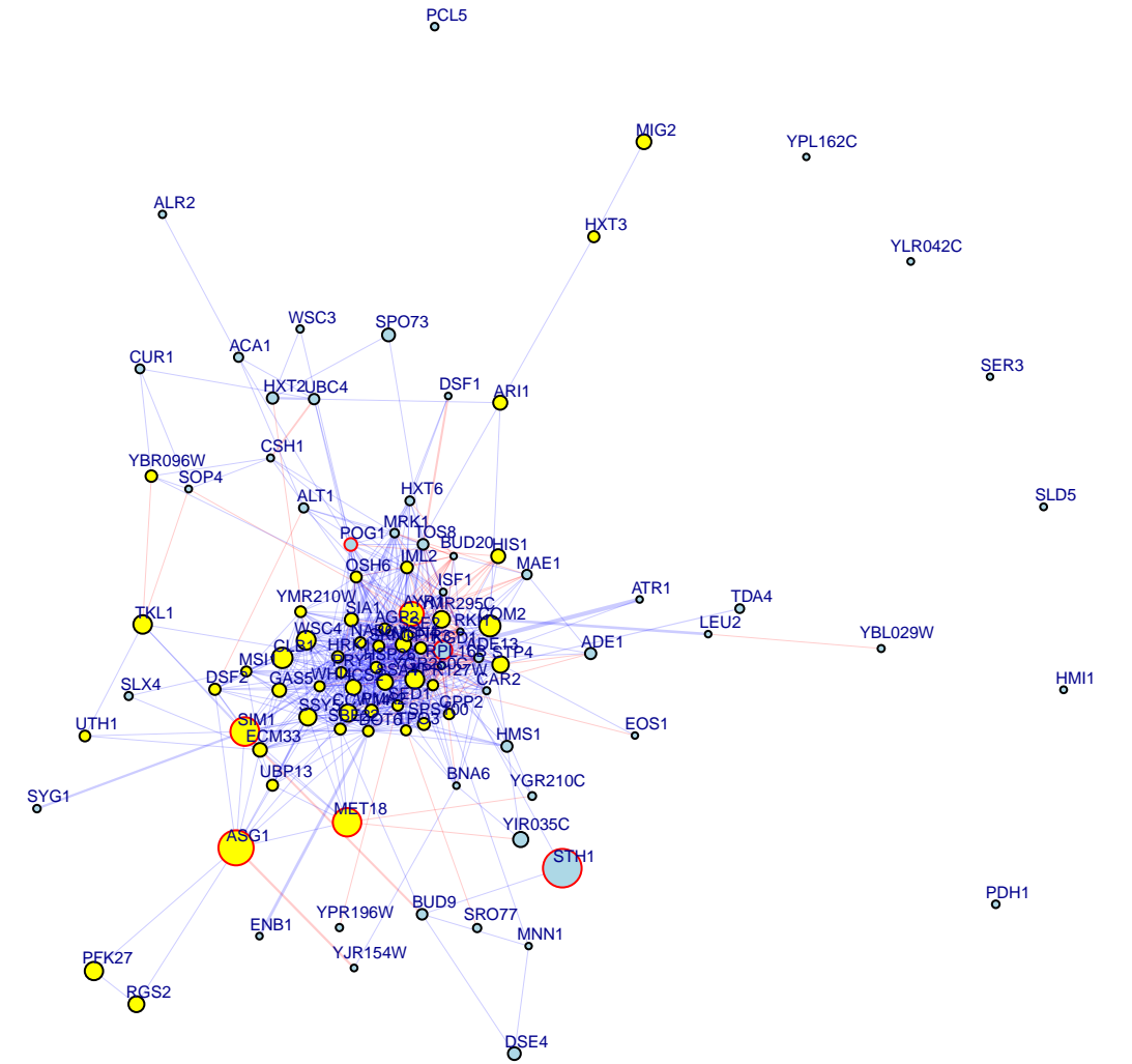
chrIX:105090_T/C top 100 up and down genes
