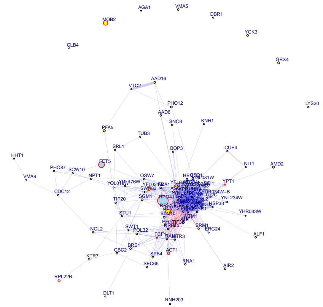
chrVI:71959_C/T top 100 up and down genes
