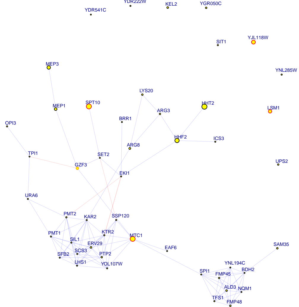
chrX:181214_T/C top 50 down genes
