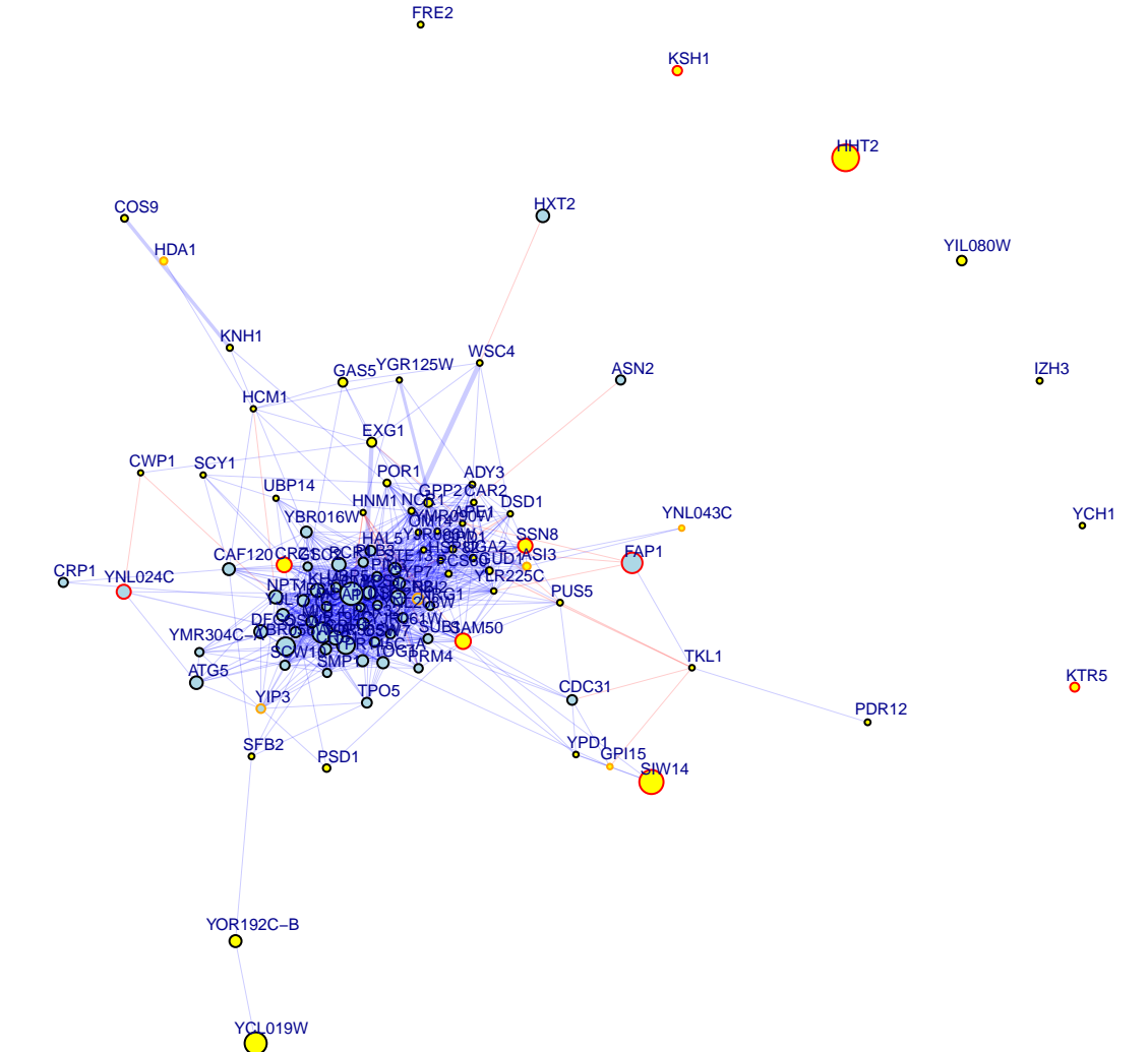
chrXIV:579945_GTТА/G top 100 up and down genes
