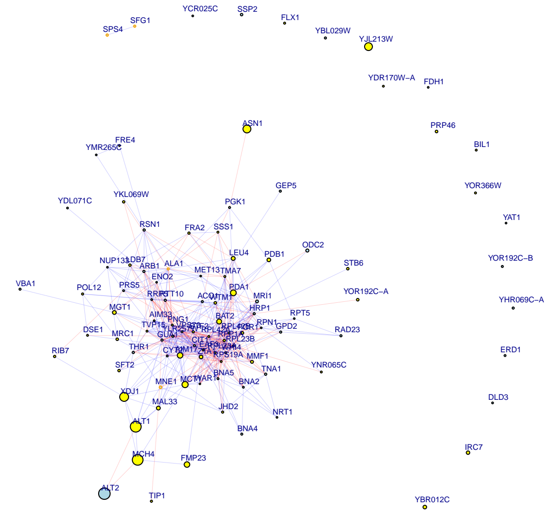
chrXV:958080_T/A top 100 up and down genes
