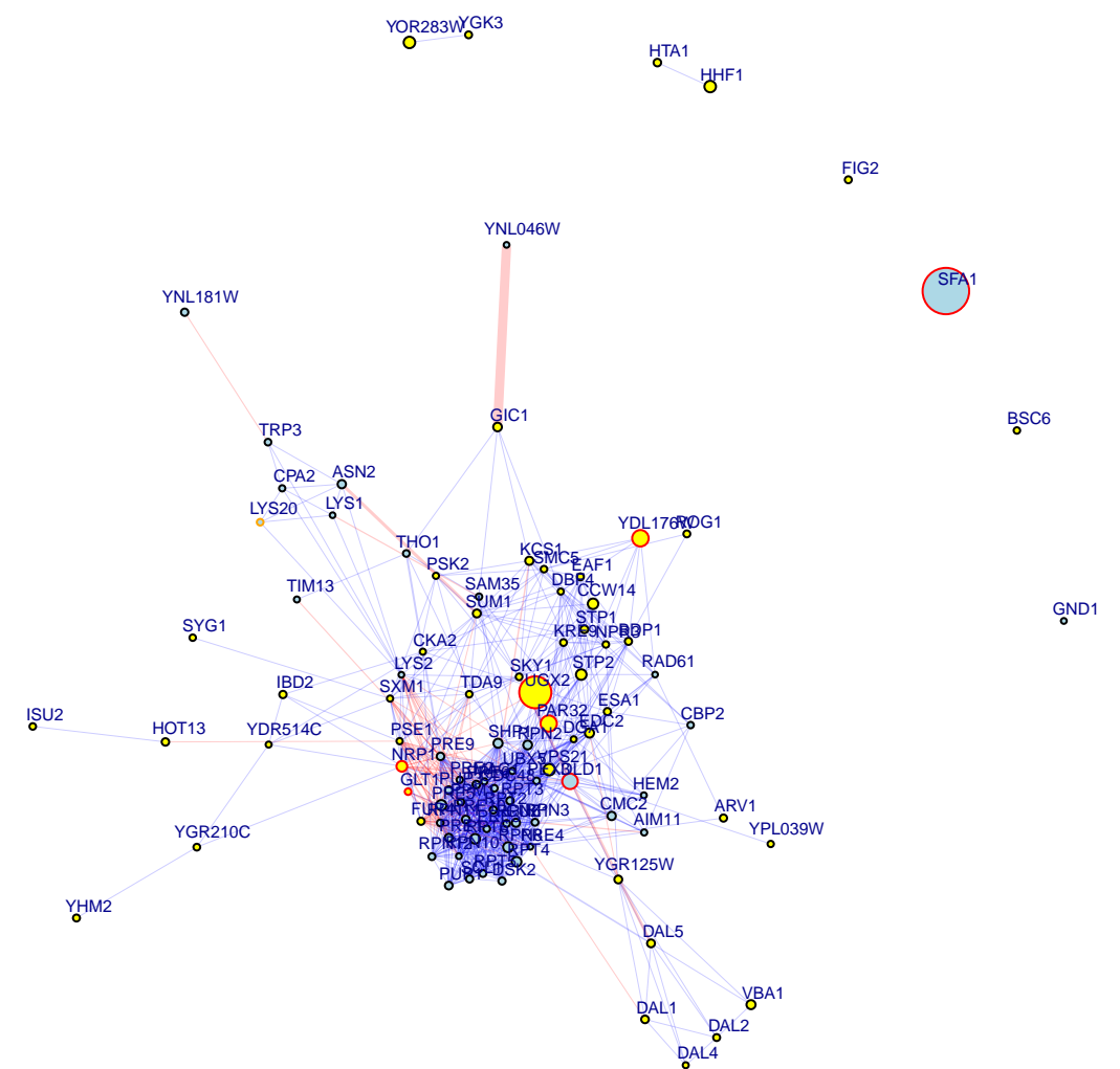
chrIV:156943_A/G top 100 up and down genes
