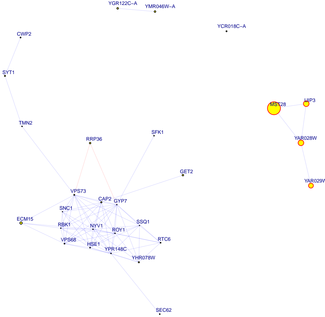
chr1:189123_C/T top 28 down genes
