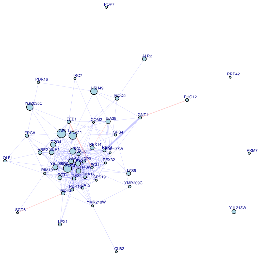
chr1:48890_C/T top 50 up genes
