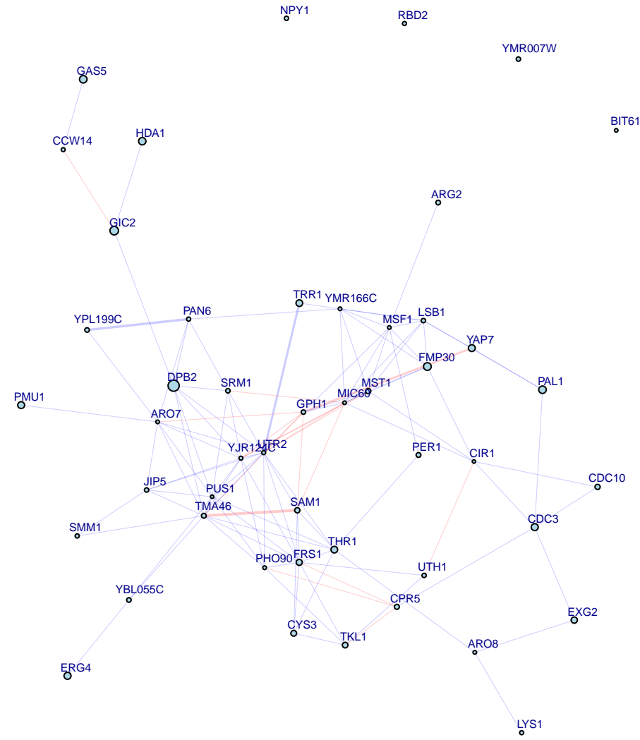
chrIX:178160_C/T top 50 up genes
