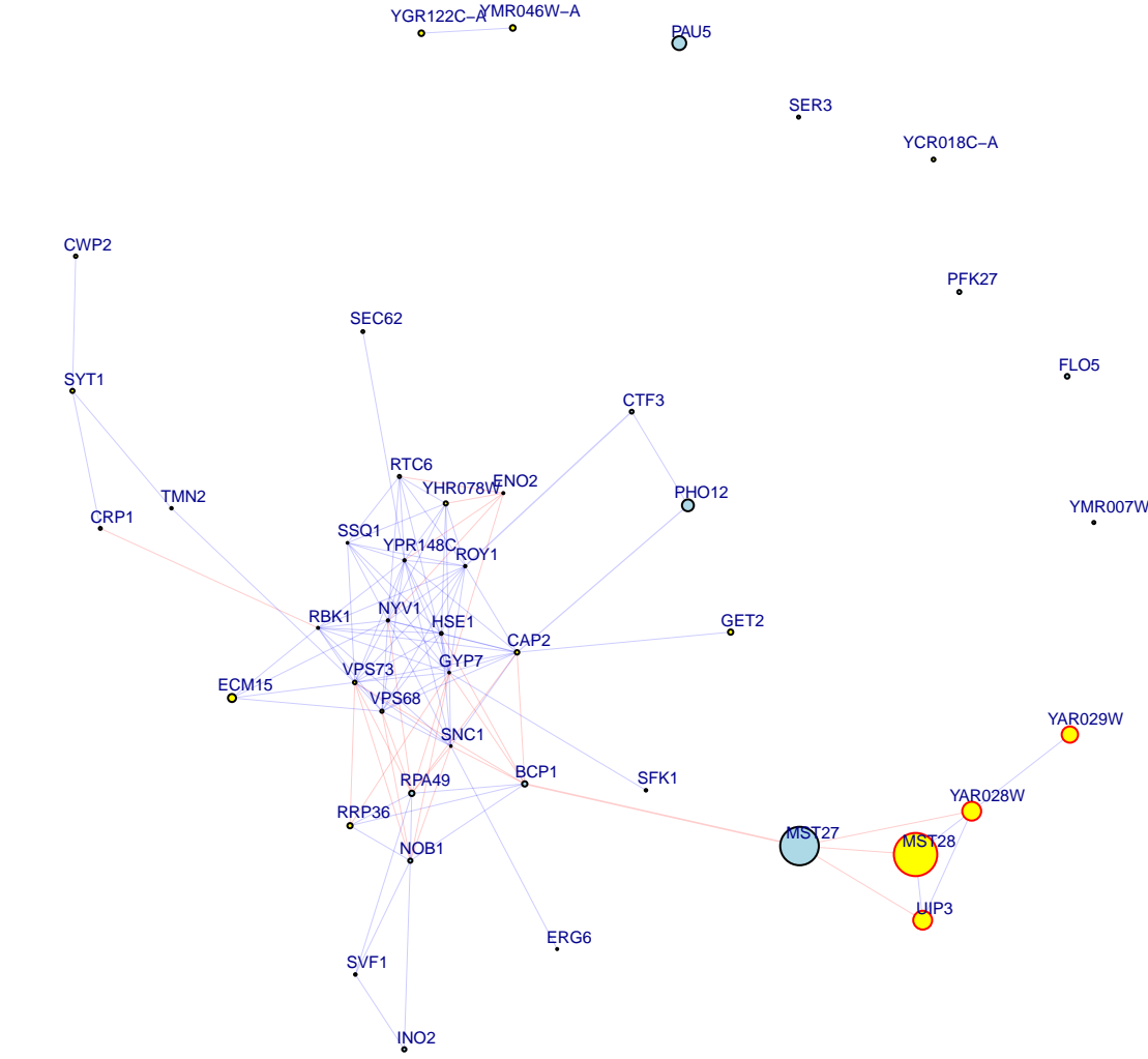
chr1:189123_C/T top 44 up and down genes
