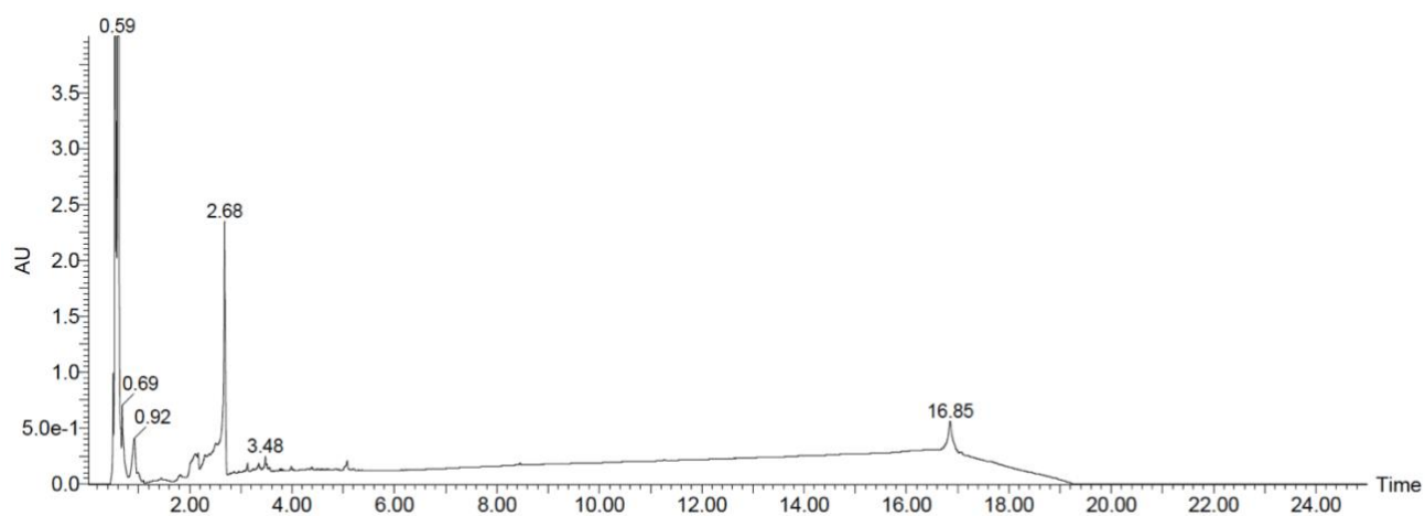
Figure S1: UHPLC - MS/ MS of crude extract of Stachys Sieboldii
