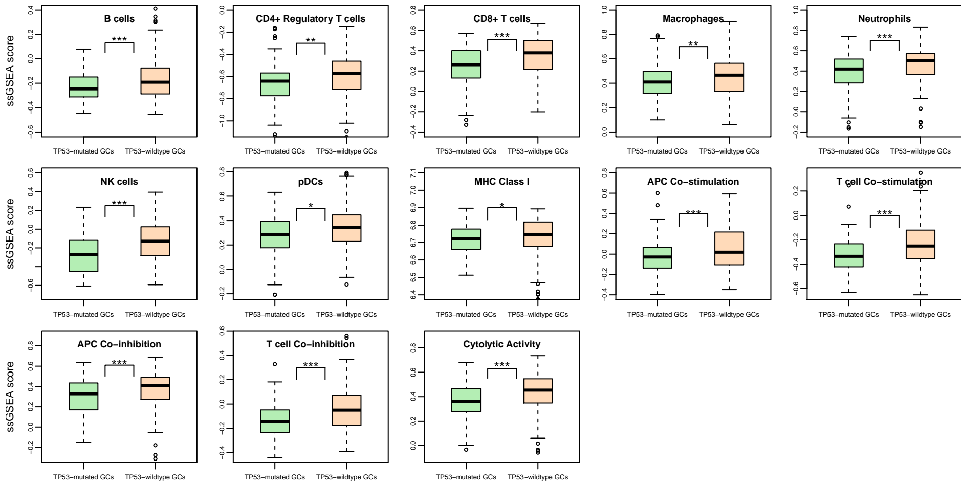
Immune cell type and function genes (ACRG)
