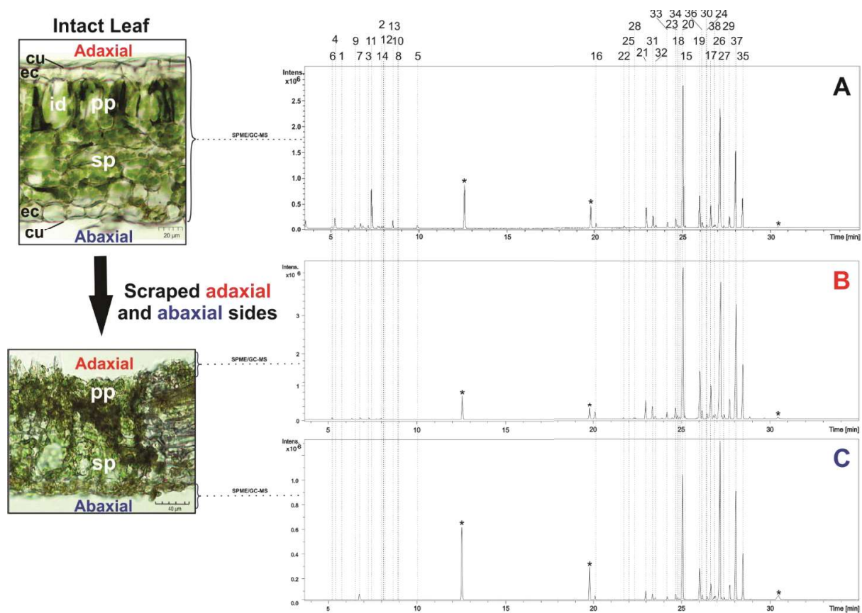
S5 Fig. SPME analysis of intact leaves and adaxial and abaxial surfaces of S7 by GC-MS. (*peak products of SPME fiber; cu: cuticle; ec: epidermal cell; id: idioblast; pp: palisade parenchyma; sp: spongy parenchyma; id: idioblast).
