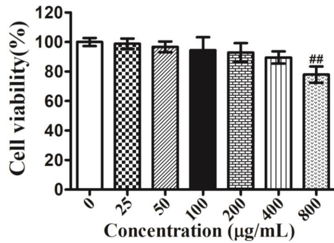
Supplemental Figure S2. Cytotoxicology of ASP in the Hep3B cell lines. The cytotoxicity test of ASP against Hep3B cells was performed by MTT assay. ## P < 0.01 compared with the “0” group.
