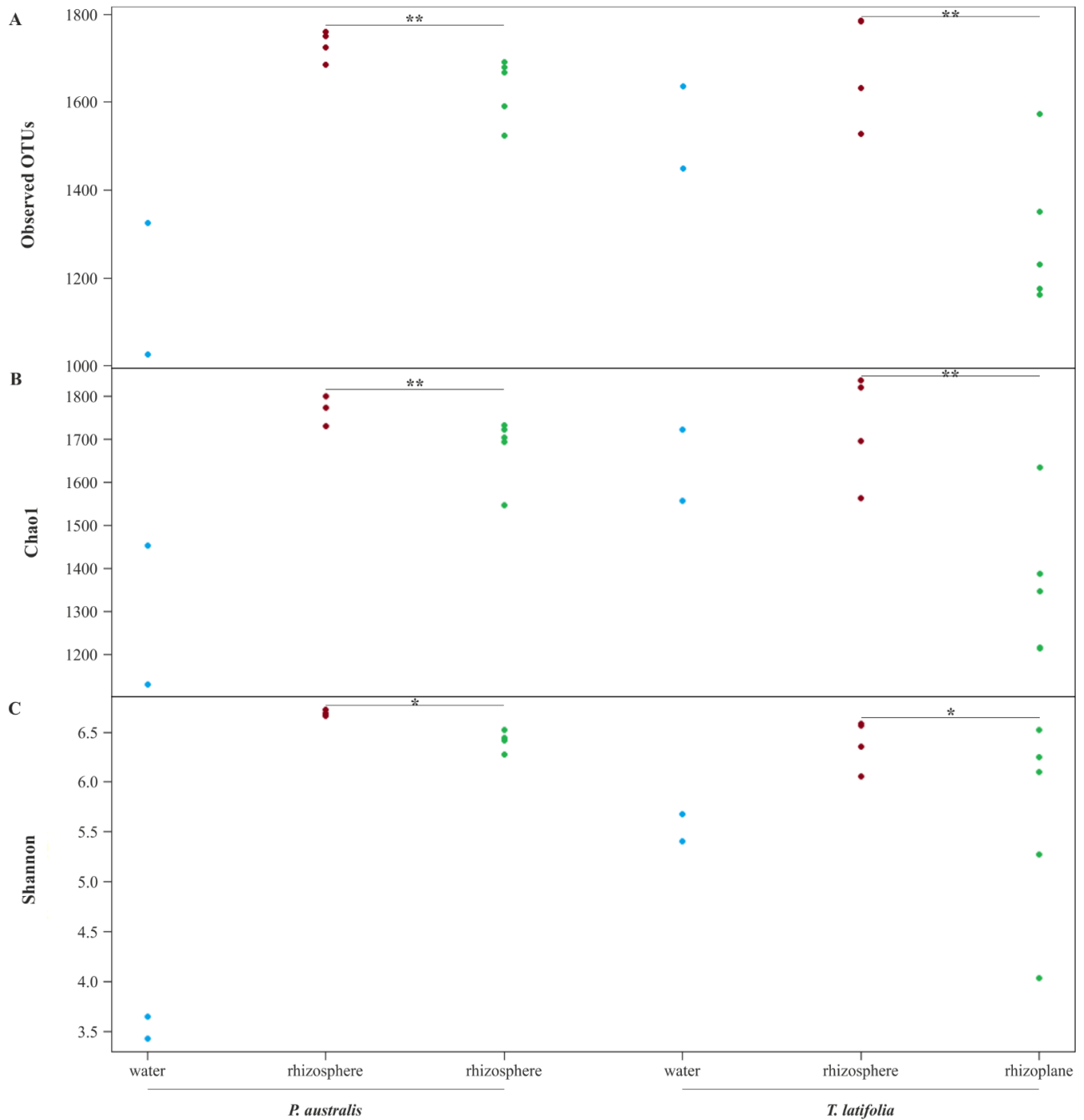
SUPPLEMENTARY FIGURE 2. Alpha diversity calculation for samples set2. OTUs richness of water, rhizosphere and rhizoplane microbiotas of Phragmites australis and Typha latifolia indicated by number of Observed OTUs (A) and by Chao1 index (B). The OTUs evenness of the two plants microbiotas is shown by Shannon index (C). Dots represent single samples. Asterisks denote statistically significant differences between rhizosphere and rhizoplane microhabitats (**P < 0.01, * P < 0.05).
