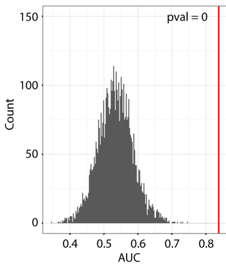
AUC Distribution of Random Signature (ICGC)
