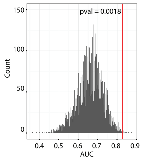
AUC Distribution of Random Signature (GSE71729)
