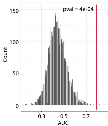
AUC Distribution of Random Signature (GSE54795)
