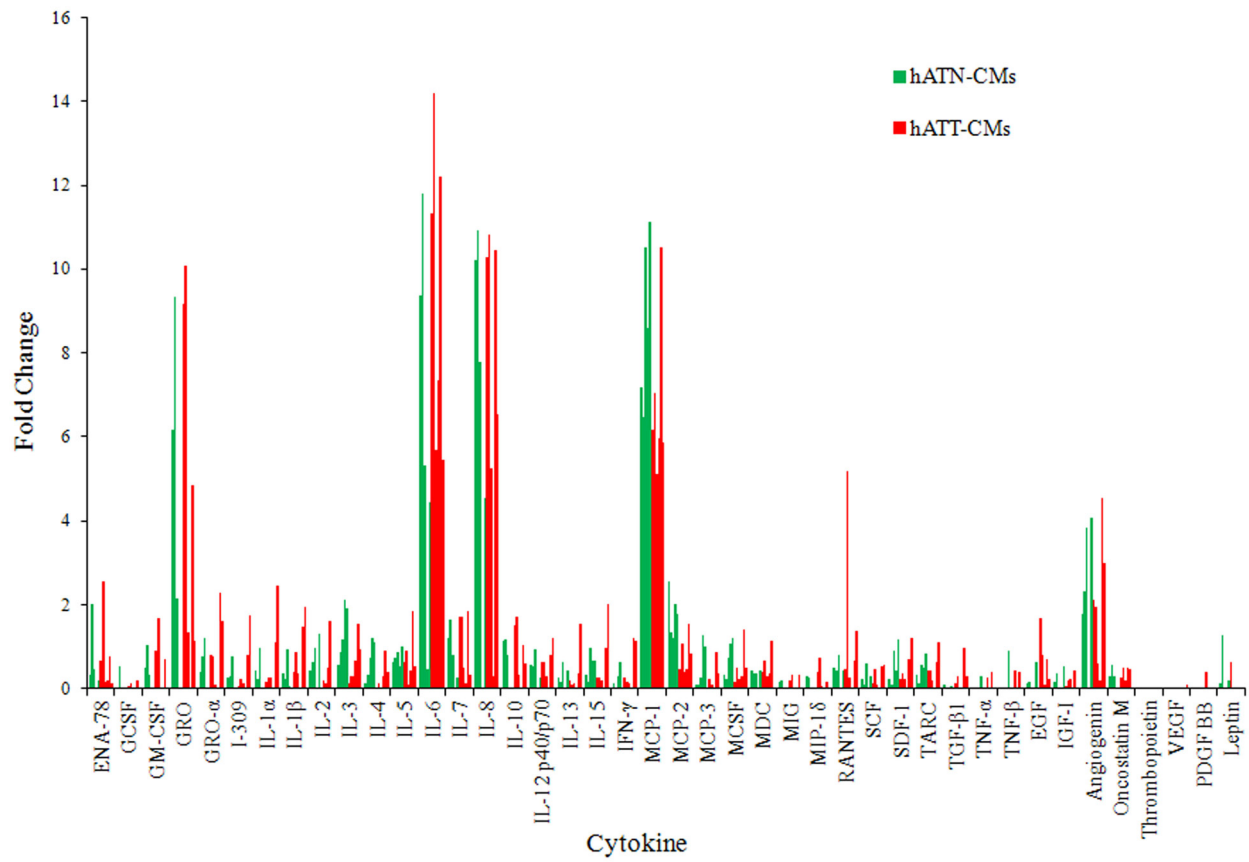
Supplementary Figure 1: Array of 42 cytokines. Dots from the array were measured by densitometry and relativized to control membrane. Bar chart shows relative fold change for each cytokines of hATN-CMs (n=5) and hATT- CMs (n=6).
