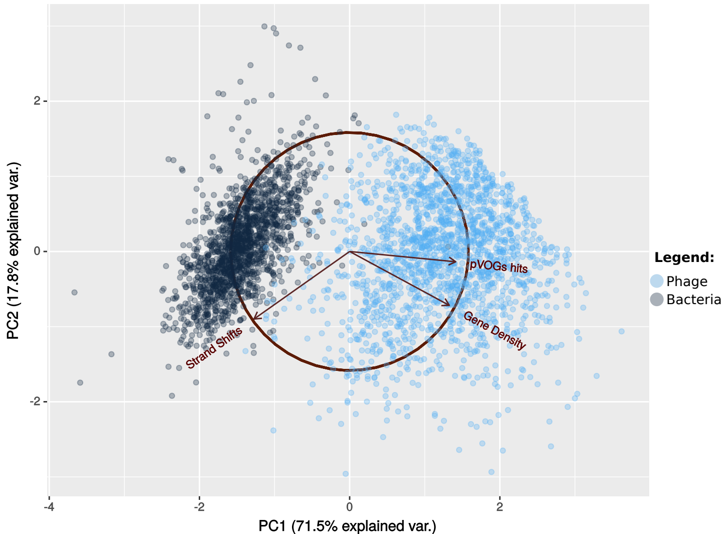
Figure S1: Principal Component Analysis using the three features implemented in MARVEL's Random Forest classifier. The first and second component explain 89% of the variation and each feature contributes proportionally to the length of its vector shown within the circle. Feature values were scaled and centered and PCA analysis was performed with pcomp() function from R.
