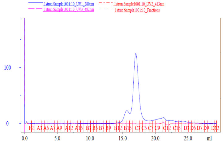
Chromatogram
