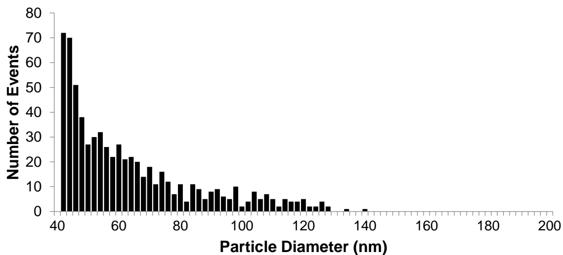
S1 Fig. Example size distribution histogram of particle diameters plotted with events detected from a single sample. Data were binned by 2 nm increments and later classified as 40-60, 60-100, or >100 nm for statistical analysis.
