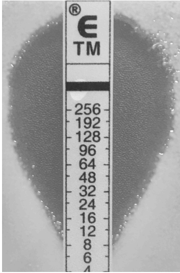
recA::Tc/vector
