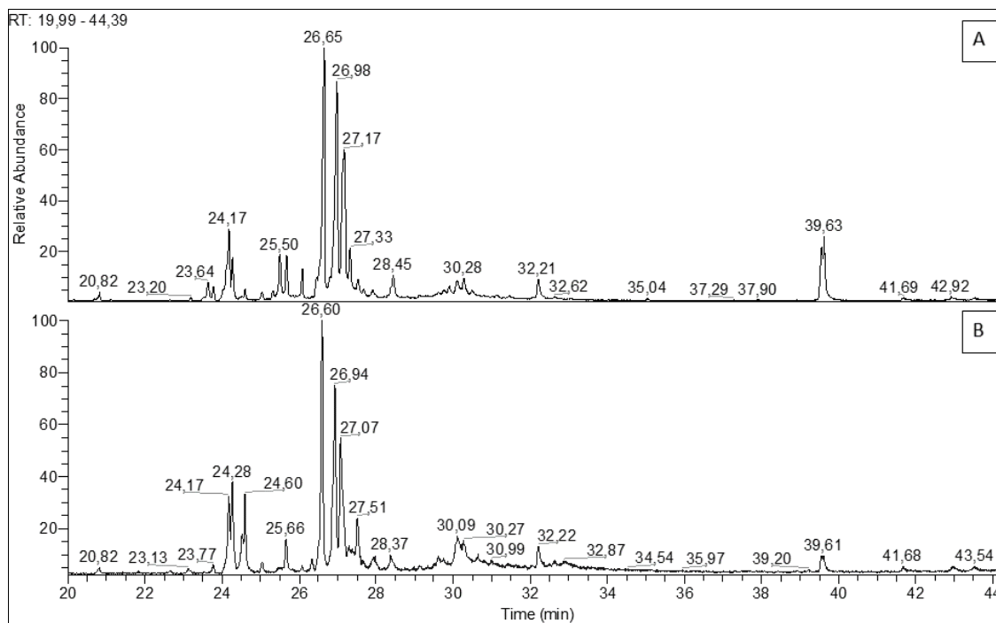
Figure S1: Chromatograms of DCME (A) and PEE (B) extracts of P. wiferum heartwood obtained by GC-MS analyses.
