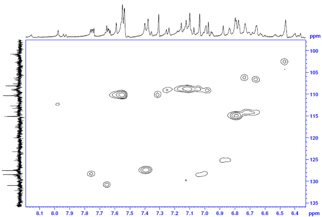
Supplementary Figure 2: HSQC spectrum of RFP A
