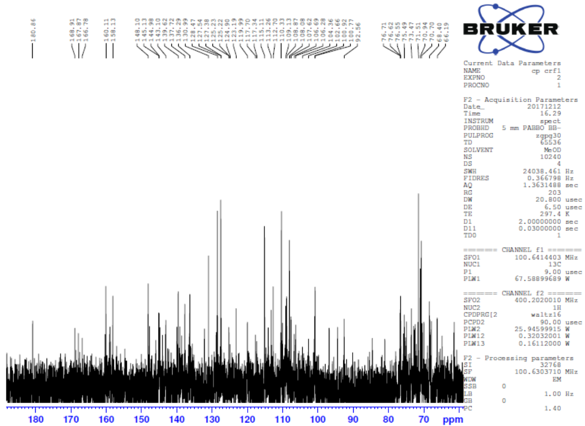
Supplementary Figure 4: 13 C spectrum of RFPA
