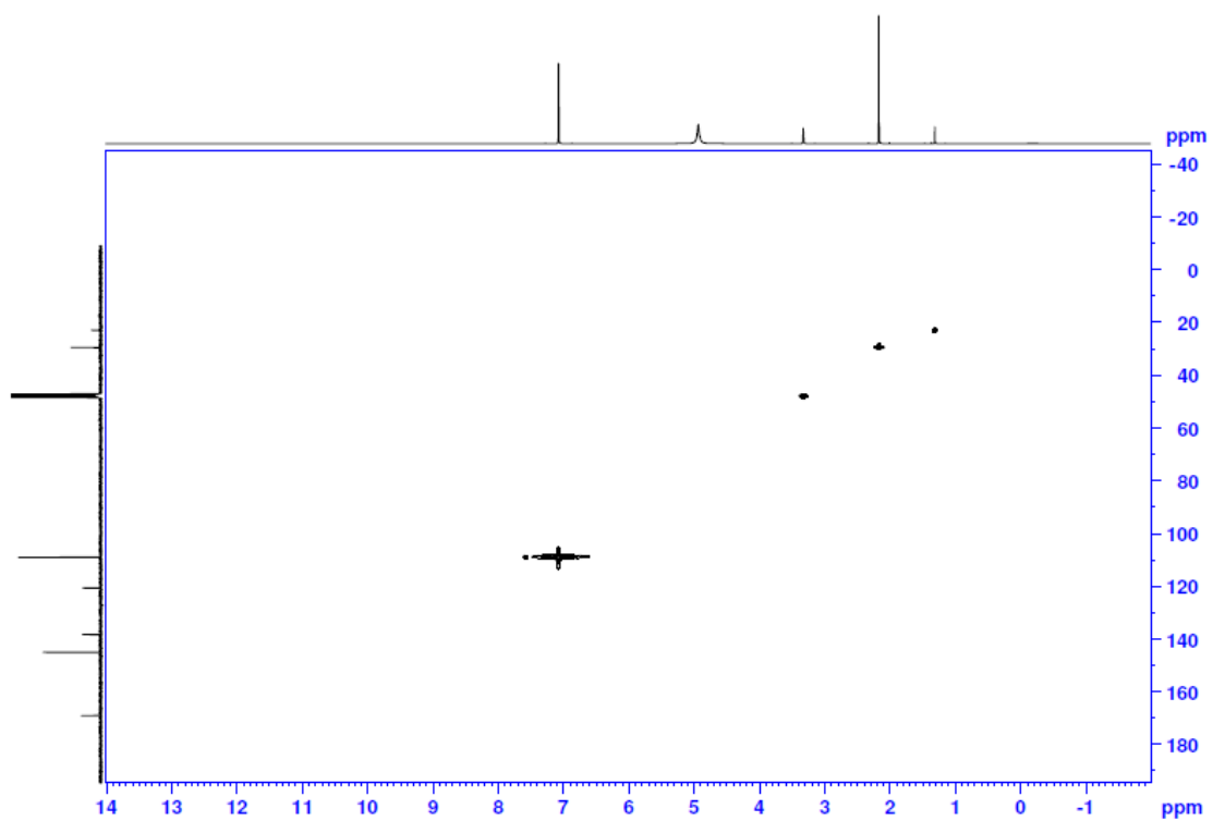
Supplementary Figure 1: HSQC spectrum of gallic acid standard
