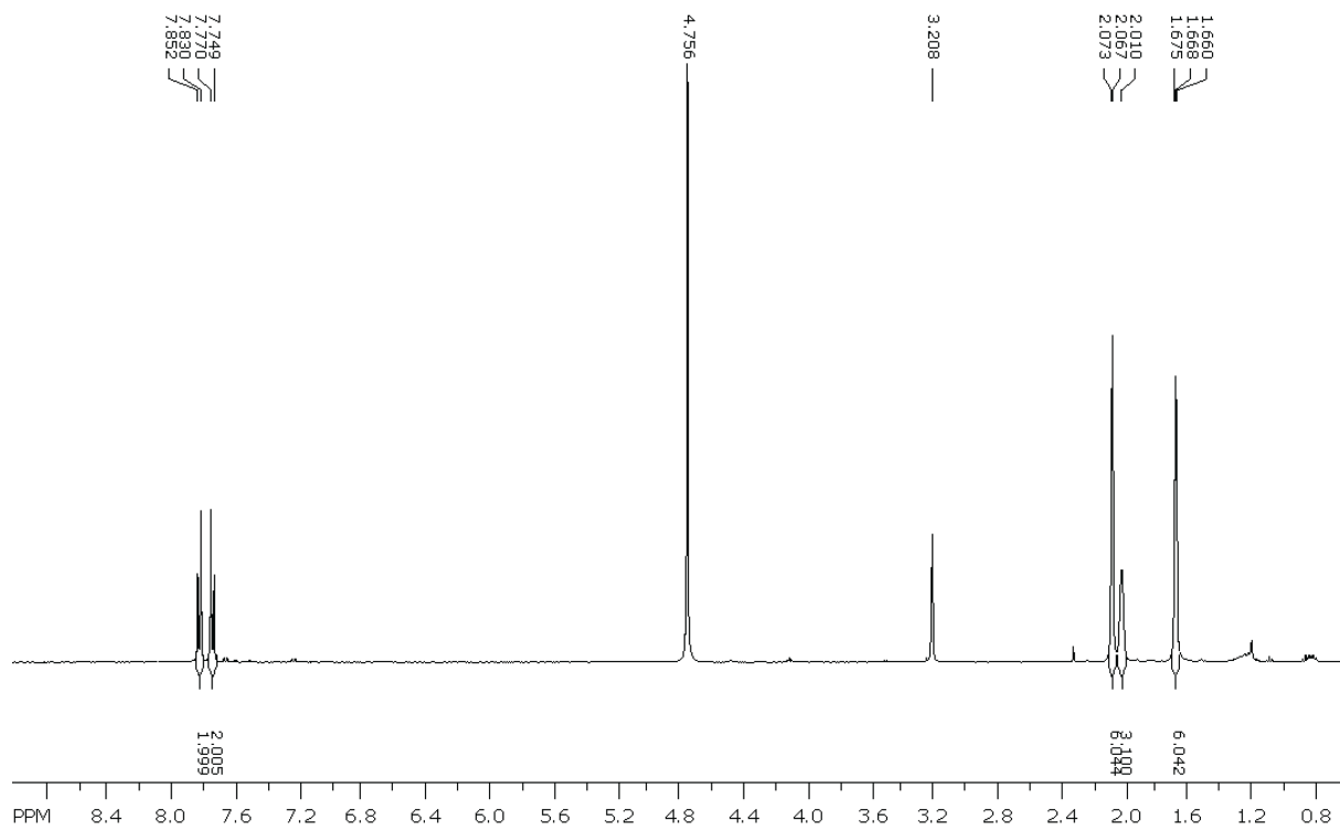
Supplementary Figure 5. ^1\text{H} -NMR of 7.
