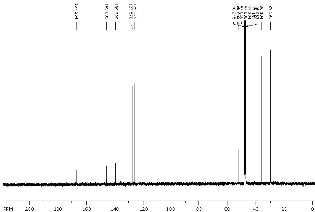
Supplementary Figure 6. 13 C-NMR of 7.
