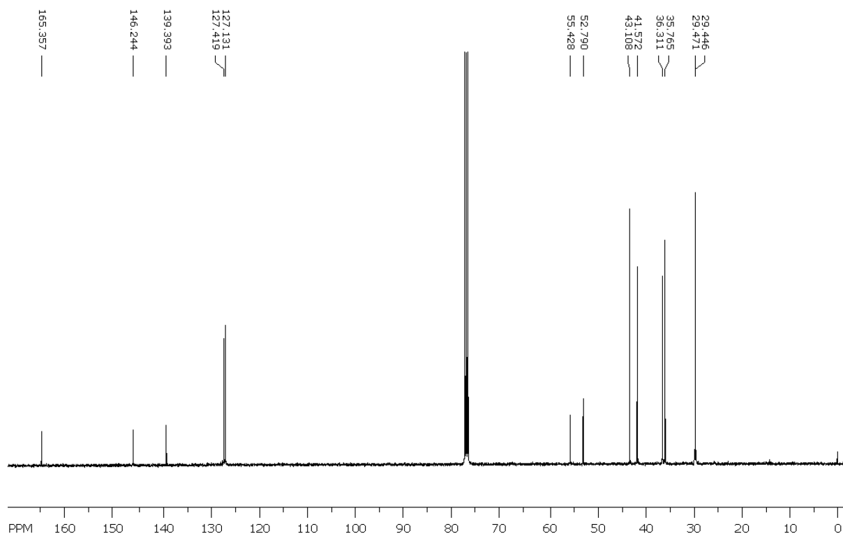
Supplementary Figure 2. 13 C-NMR of 3.
