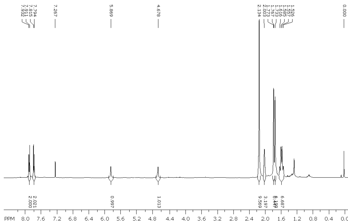
Supplementary Figure 1. 1 H-NMR of 3.
