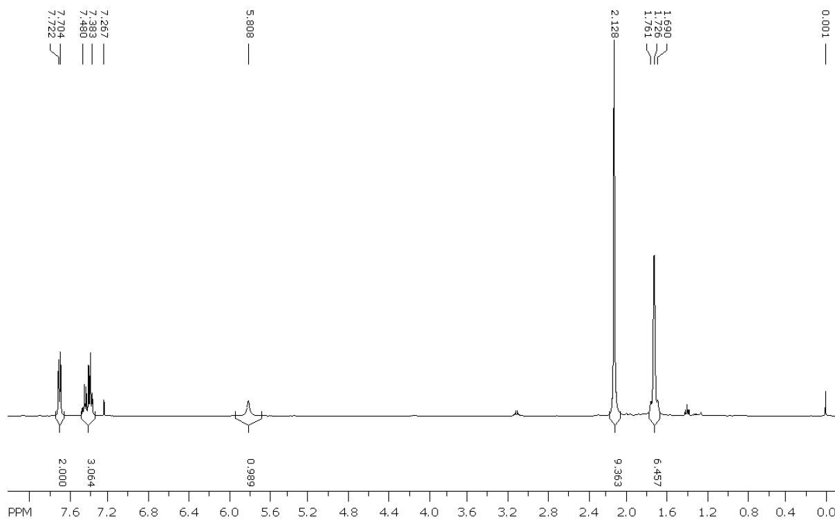
Supplementary Figure 3. 1 H-NMR of 6.
