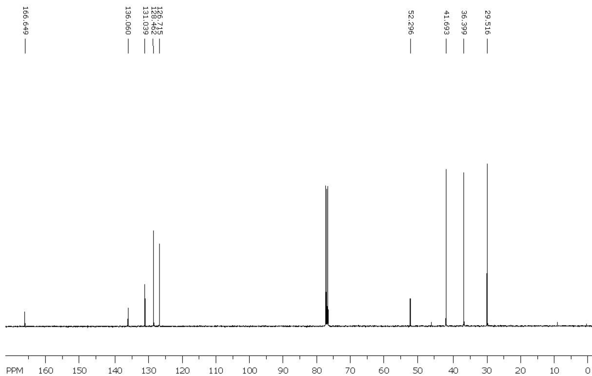
Supplementary Figure 4. ^{13}\text{C} -NMR of 6.
