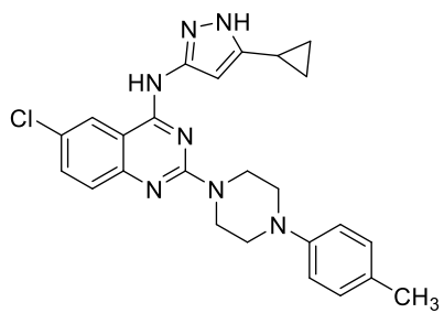
Compound 7b
