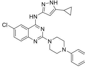
Compound 7a
