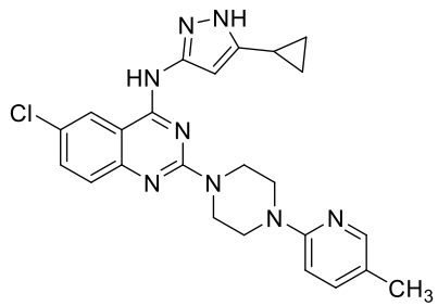
Compound 8c
