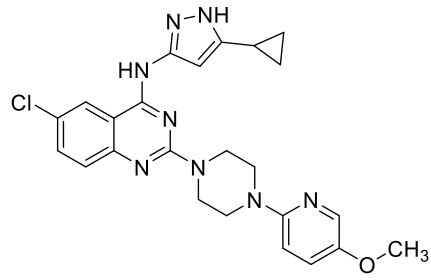
Compound 8b
