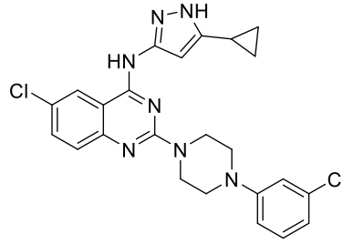
Compound 7f
