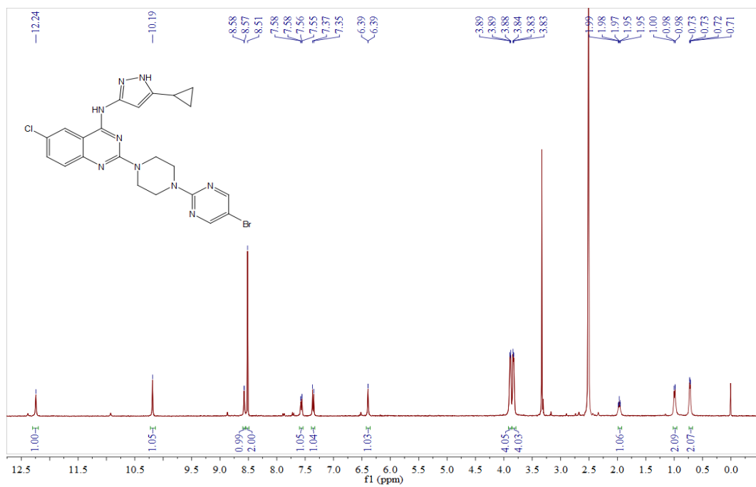
Compound 9c
