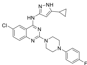
Compound 7i
