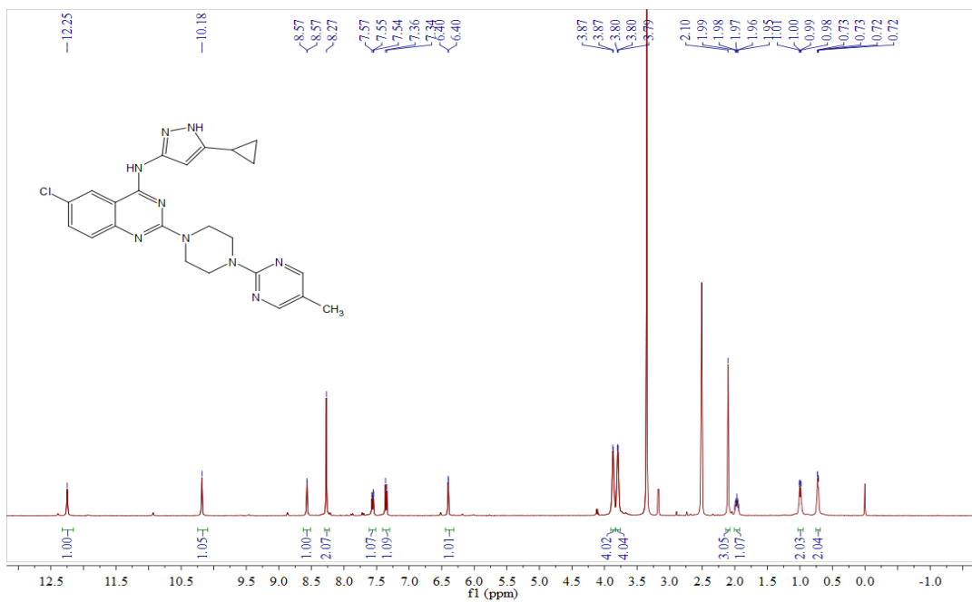
Compound 9b
