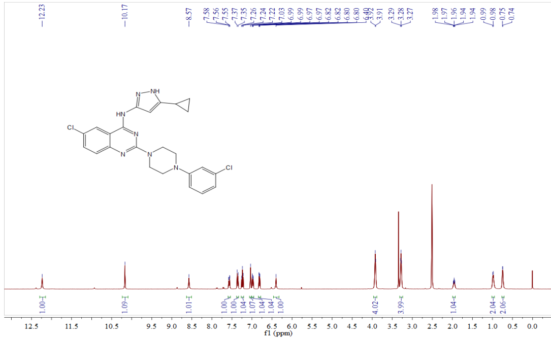
Compound 7f
