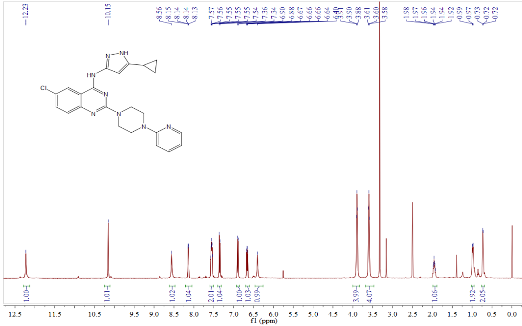
Compound 8a
