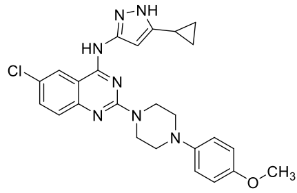
Compound 7g
