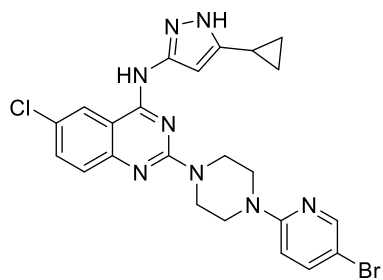
Compound 8d
