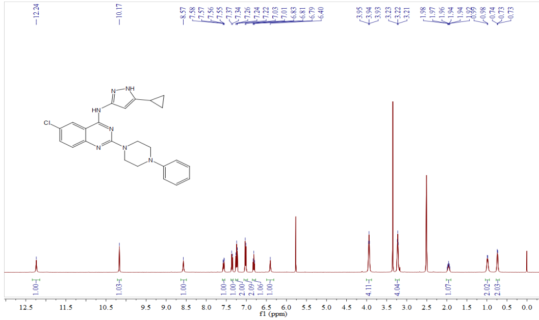
Compound 7a
