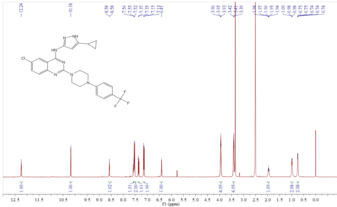
Compound 7d
