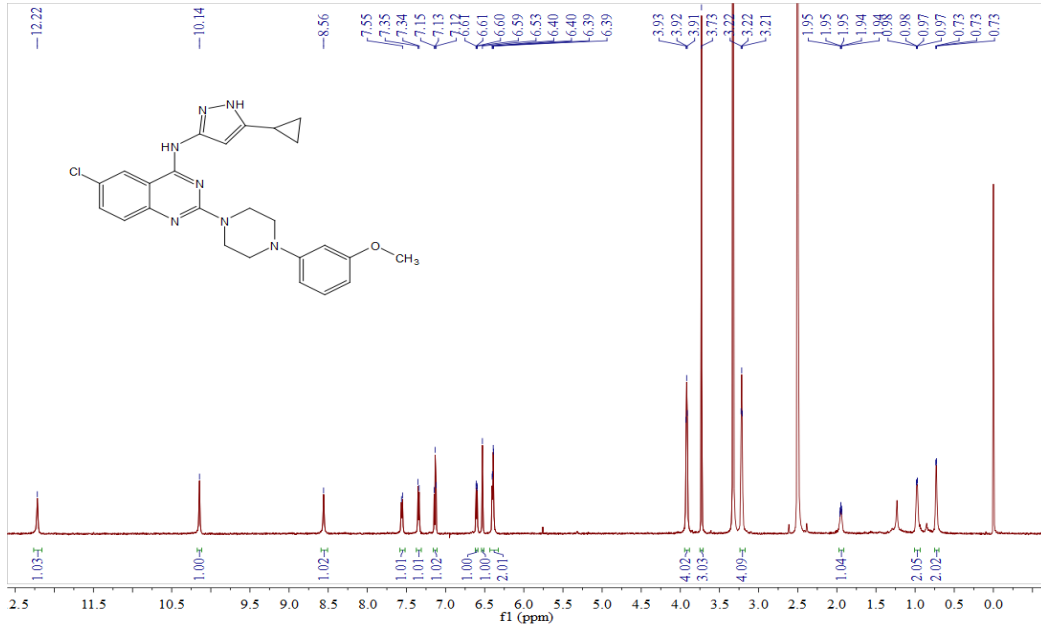
Compound 7h
