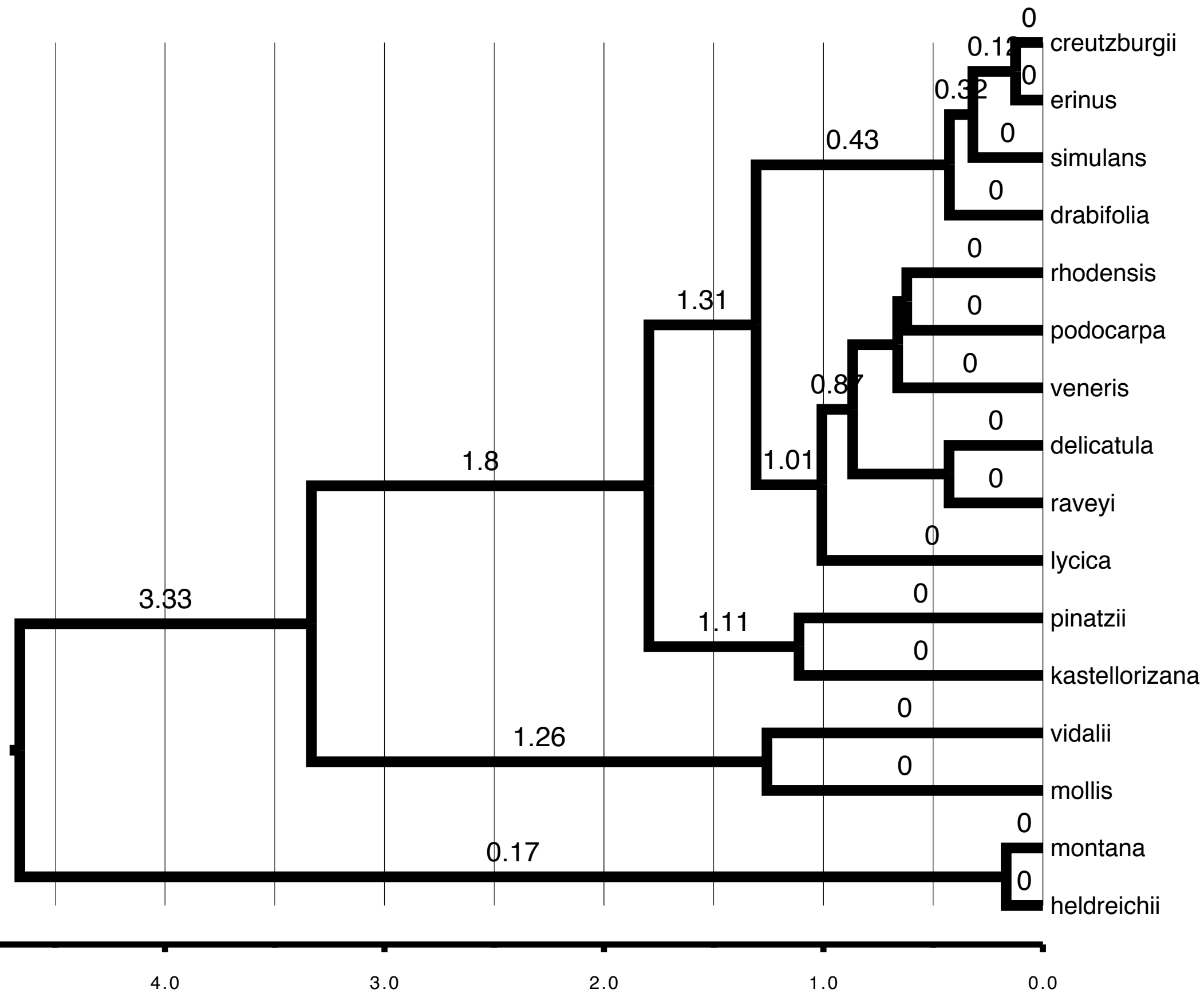
Fig. S5 Chronogram inferred using a coalescent species tree approach in *BEAST. Results from this analysis provided divergence dates an order of magnitude younger than other methods and previous studies of the group. Numbers above branches are divergence dates in millions of years ago.
