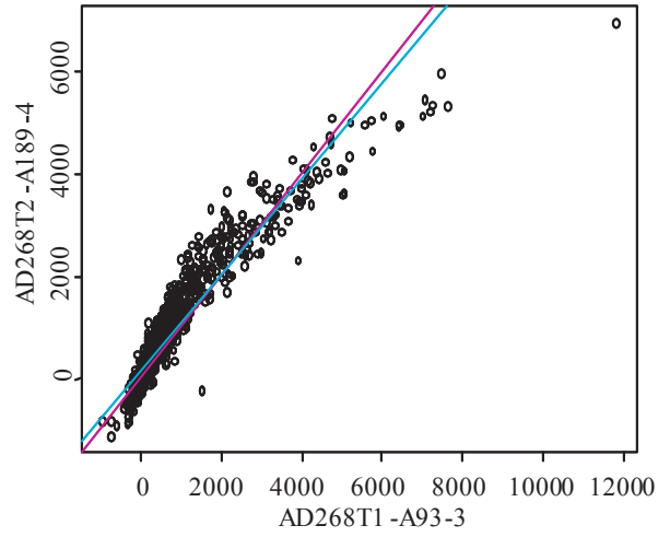
Linear scaling, 2% trimmed mean of "P" genes
