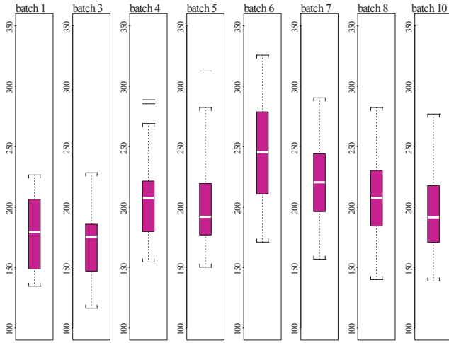
Linear scaling, 2% trimmed mean of "P" genes
