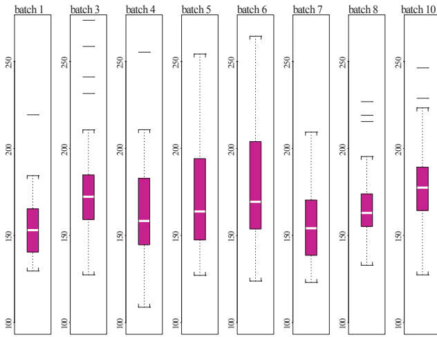
Nonlinear rank invariant scaling, 2% trimmed mean of "P" genes
